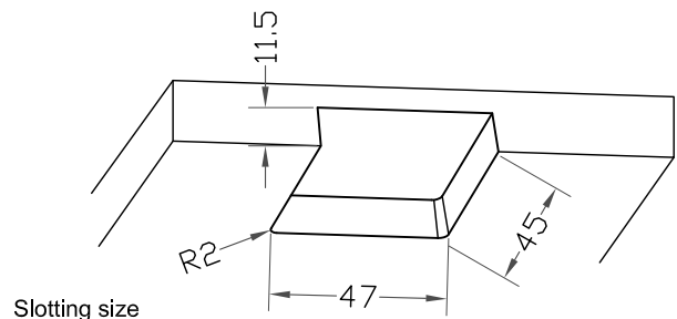
Slotting size
