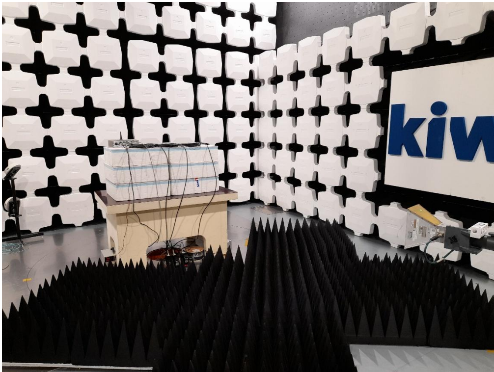
1.5 Radiated emissions measurement 18 - 26 GHz
