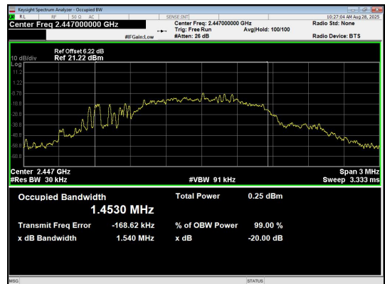
GFSK_Frequency_2447MHz
