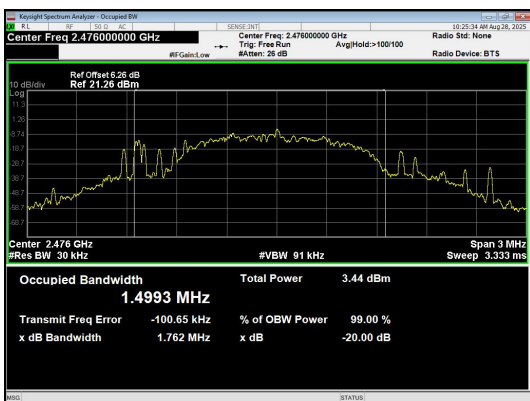
GFSK_Frequency_2476MHz
