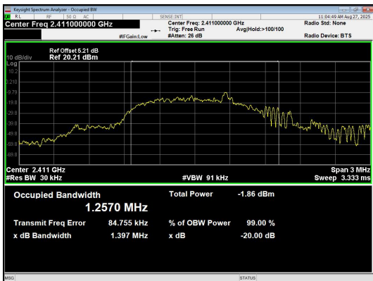
GFSK_Frequency_2411MHz
