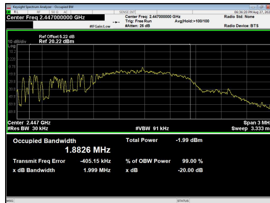
GFSK_Frequency_2447MHz
