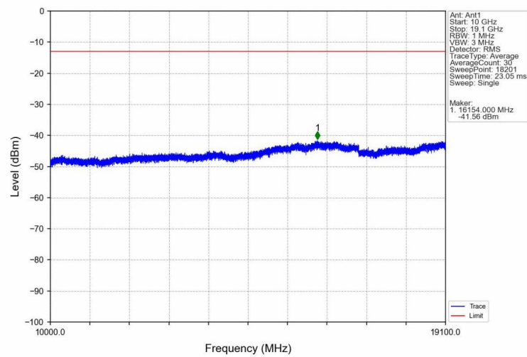
Band2_HSDPA_MCH_1880MHz_Subtest 1_NTNV
