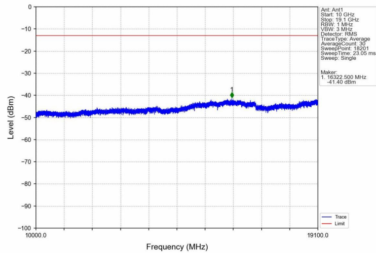
Band2_HSDPA_HCH_1907.6MHz_Subtest 1_NTNV
