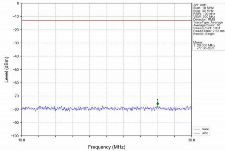
Band2_15MHz_16QAM_HCH_1902.5MHz_RB_1_0_NTNV
