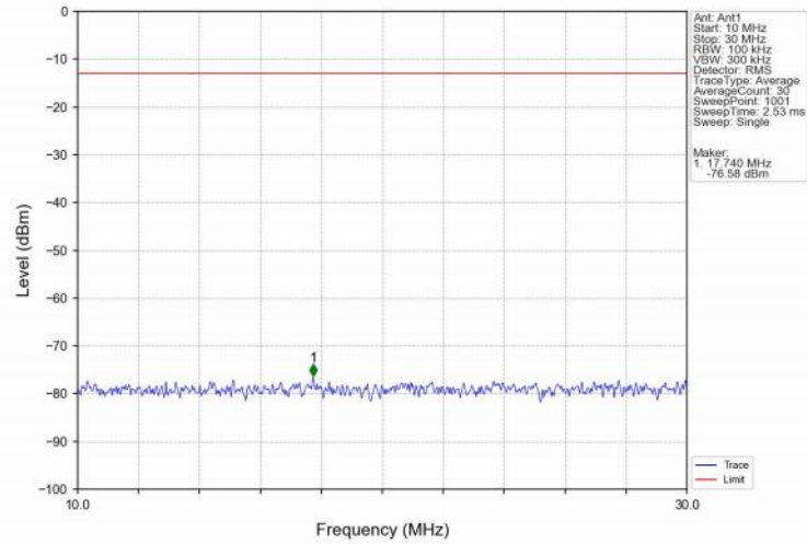
Band2_5MHz_16QAM_LCH_1852.5MHz_RB_1_0_NTNV
