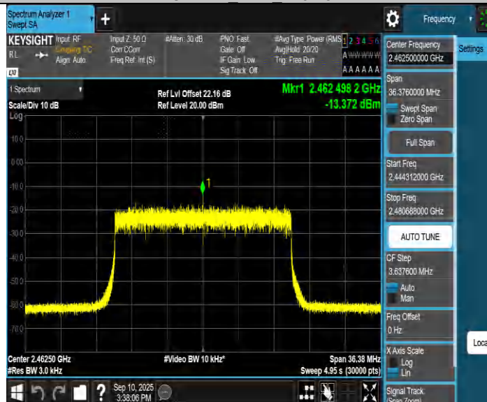
OTHER Ant2 2462.5
