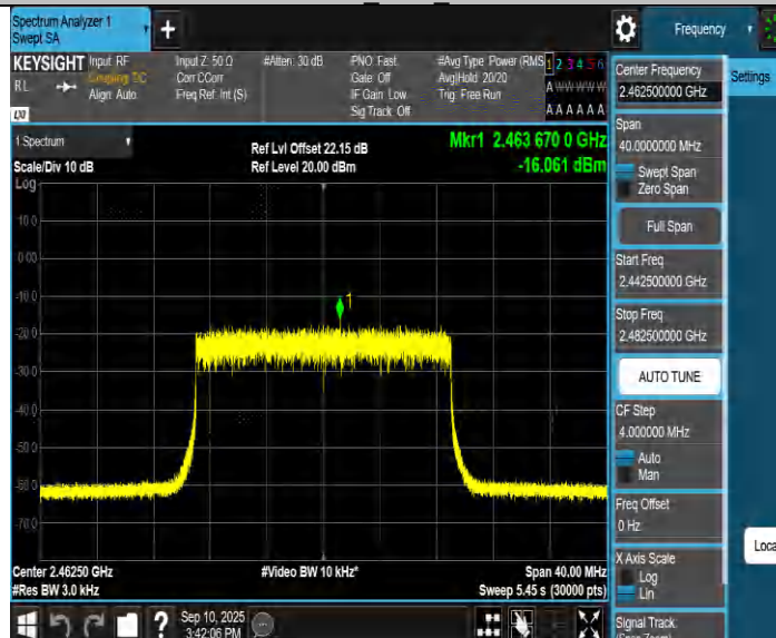
OTHER Ant2 2462.5
