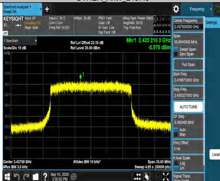
OTHER Ant1 2437.5
