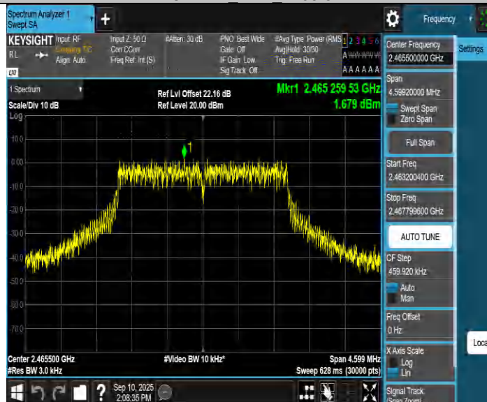
OTHER Ant2 2465.5
