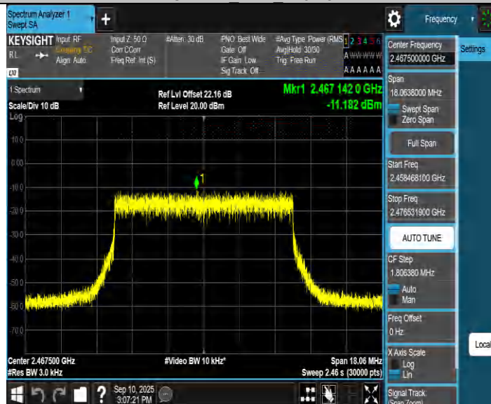
OTHER Ant2 2467.5
