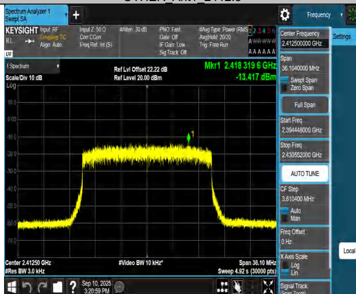
OTHER Ant2 2412.5
