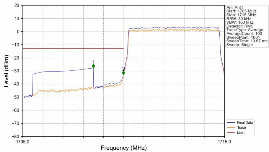
Band66_5MHz_QPSK_LCH_1712.5MHz_RB_25_0_NTNV
