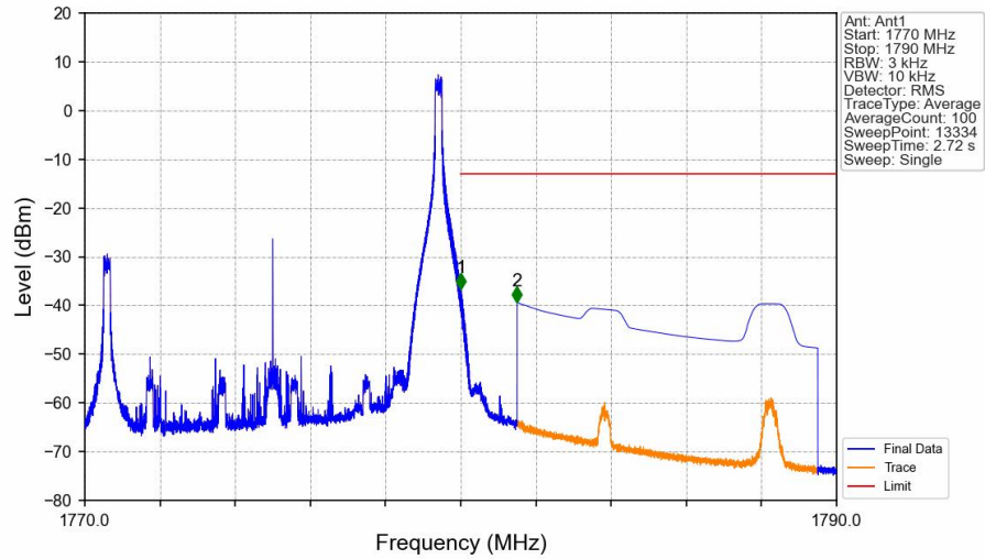
Band66_10MHz_16QAM_HCH_1775MHz_RB_1_49_NTNV
