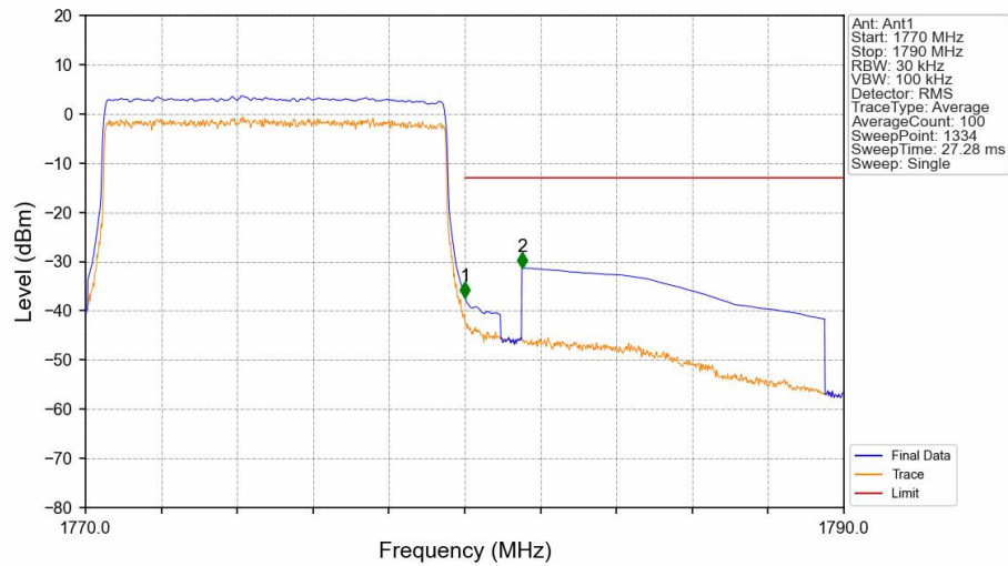
Band66_10MHz_QPSK_HCH_1775MHz_RB_50_0_NTNV
