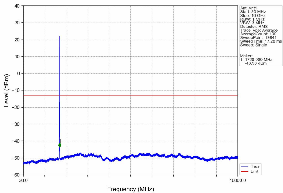
Band66_5MHz_16QAM_LCH_1712.5MHz_RB_1_0_NTNV
