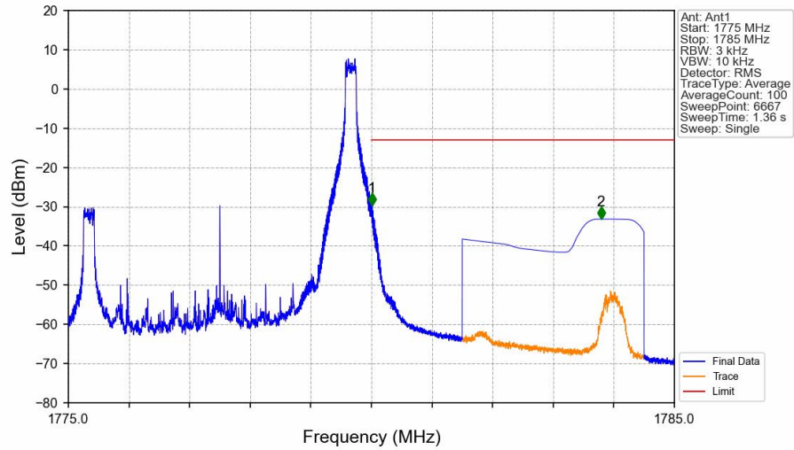
Band66_5MHz_16QAM_HCH_1777.5MHz_RB_1_24_NTNV
