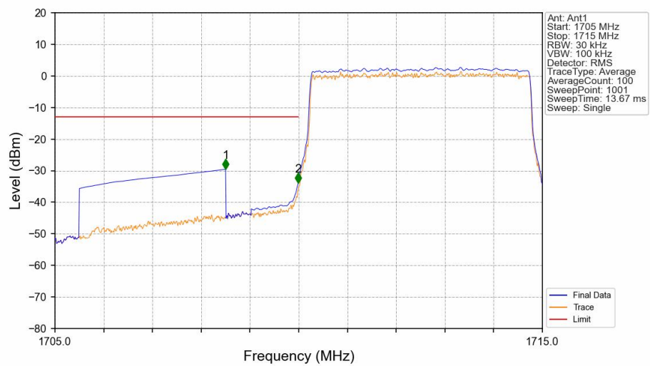
Band66_5MHz_16QAM_LCH_1712.5MHz_RB_25_0_NTNV
