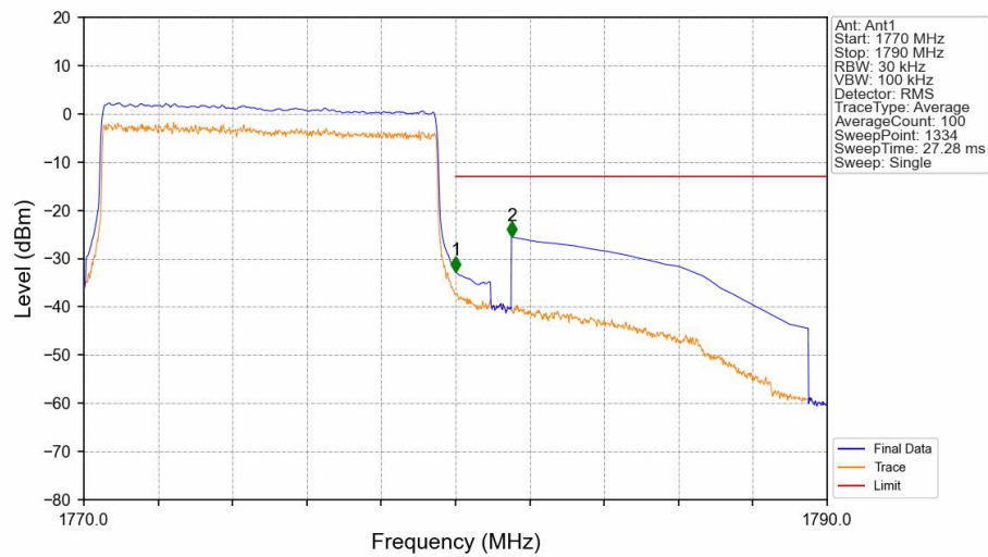
Band66_10MHz_16QAM_HCH_1775MHz_RB_50_0_NTNV
