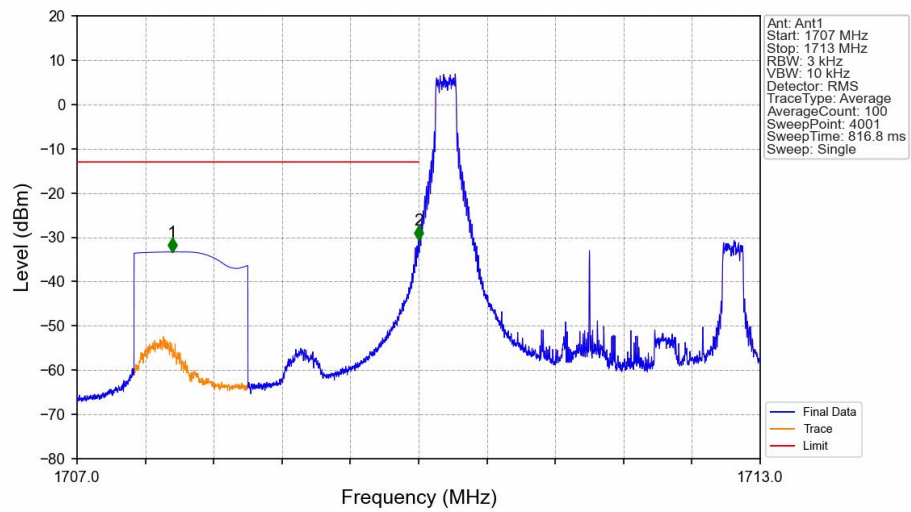
Band66_3MHz_16QAM_LCH_1711.5MHz_RB_1_0_NTNV
