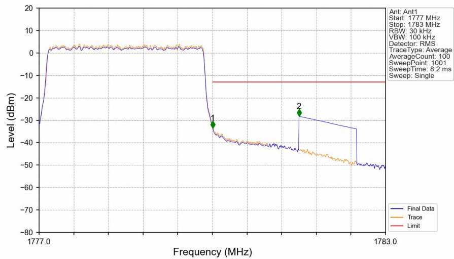
Band66_3MHz_16QAM_HCH_1778.5MHz_RB_15_0_NTNV
