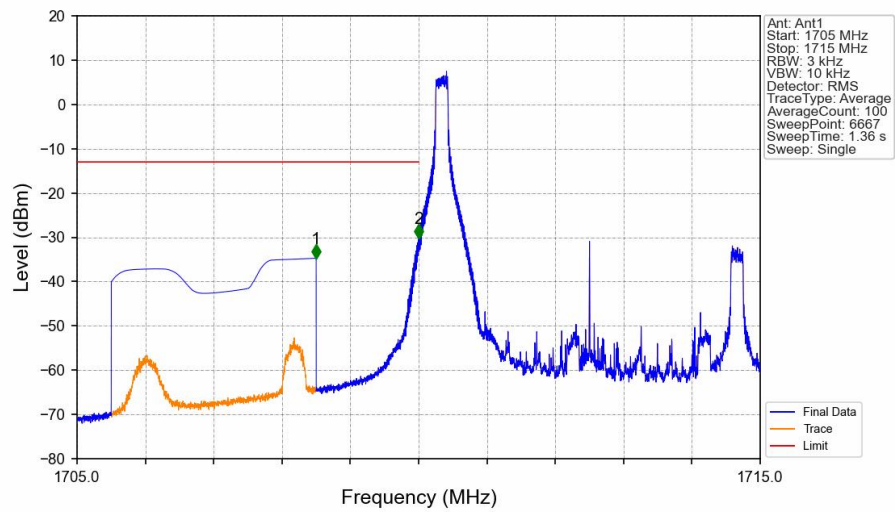
Band66_5MHz_16QAM_LCH_1712.5MHz_RB_1_0_NTNV
