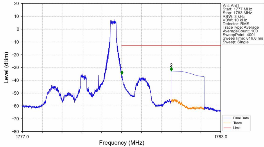
Band66_1.4MHz_16QAM_HCH_1779.3MHz_RB_1_5_NTNV
