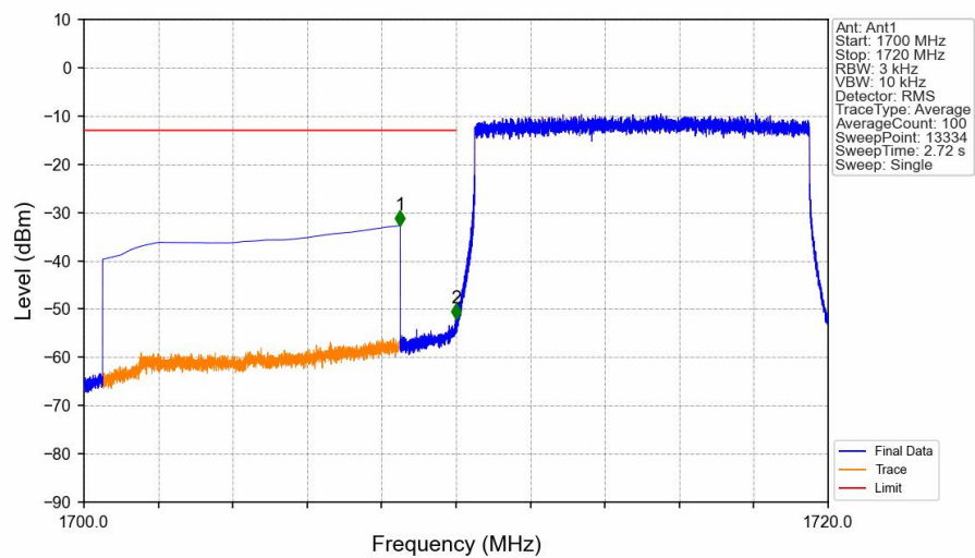
Band66_10MHz_16QAM_LCH_1715MHz_RB_1_0_NTNV
