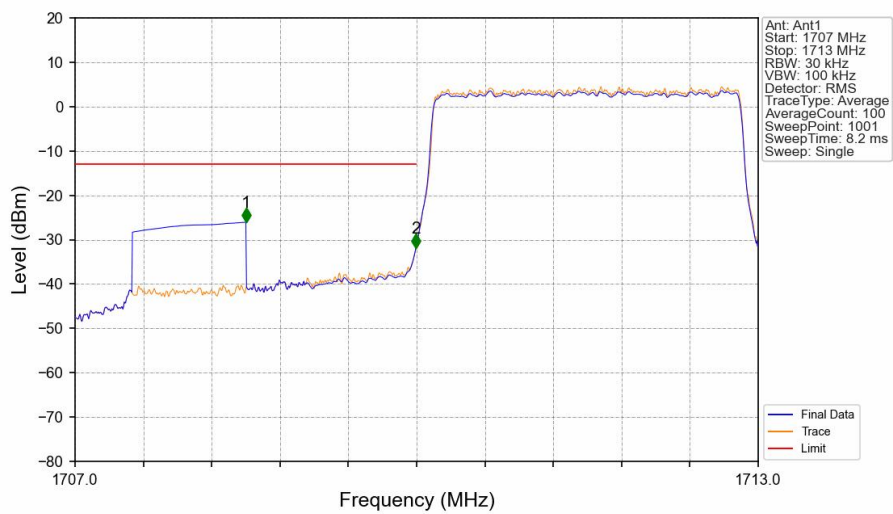
Band66_3MHz_QPSK_LCH_1711.5MHz_RB_15_0_NTNV
