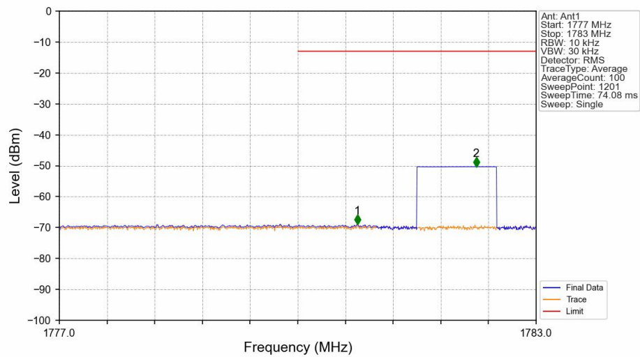
Band66_1.4MHz_16QAM_HCH_1779.3MHz_RB_6_0_NTNV
