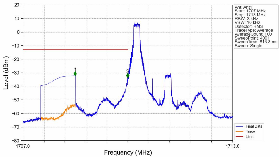
Band66_1.4MHz_16QAM_LCH_1710.7MHz_RB_1_0_NTNV
