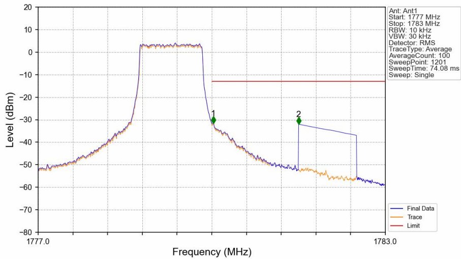
Band66_1.4MHz_QPSK_HCH_1779.3MHz_RB_6_0_NTNV
