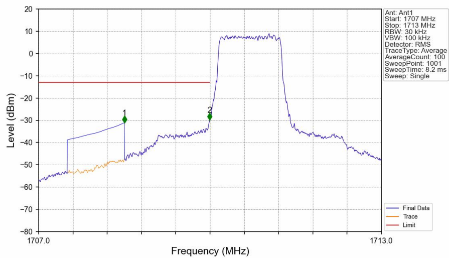
Band66_1.4MHz_QPSK_LCH_1710.7MHz_RB_6_0_NTNV
