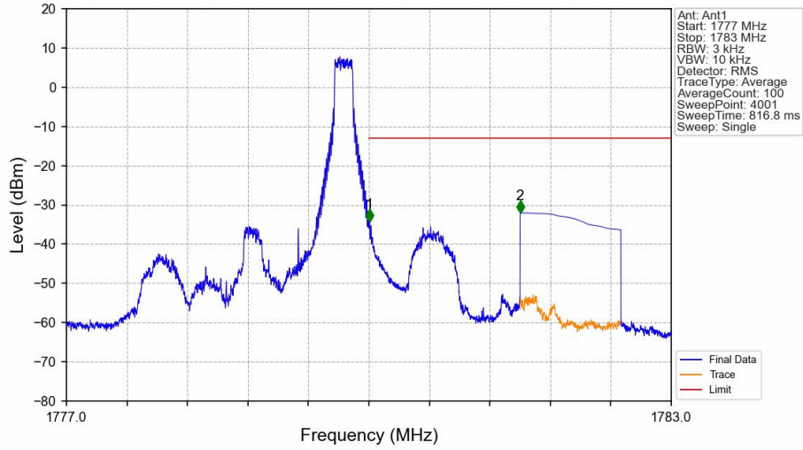
Band66_1.4MHz_QPSK_HCH_1779.3MHz_RB_1_5_NTNV
