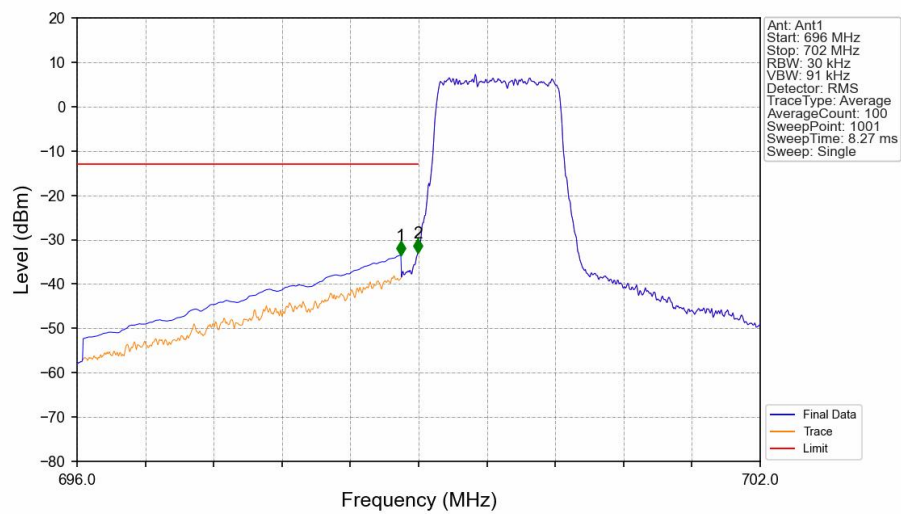
Band12_1.4MHz_16QAM_LCH_699.7MHz_RB_6_0_NTNV
