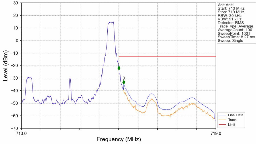
Band12_3MHz_16QAM_HCH_714.5MHz_RB_1_14_NTNV
