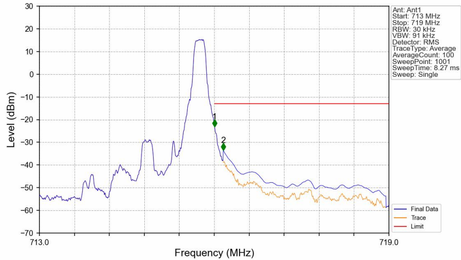
Band12_1.4MHz_QPSK_HCH_715.3MHz_RB_1_5_NTNV
