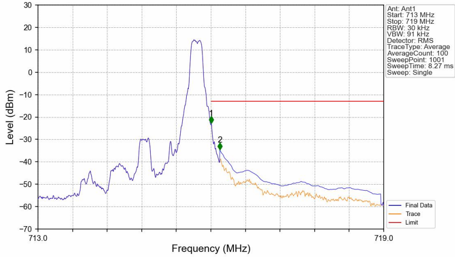
Band12_1.4MHz_16QAM_HCH_715.3MHz_RB_1_5_NTNV
