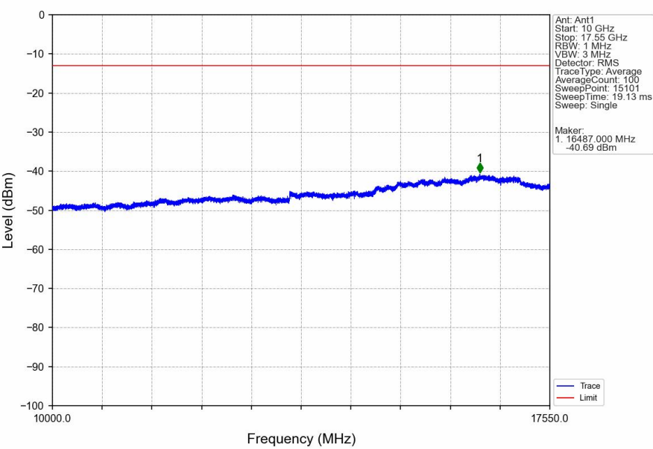
Band4_5MHz_QPSK_HCH_1752.5MHz_RB_1_0_NTNV
