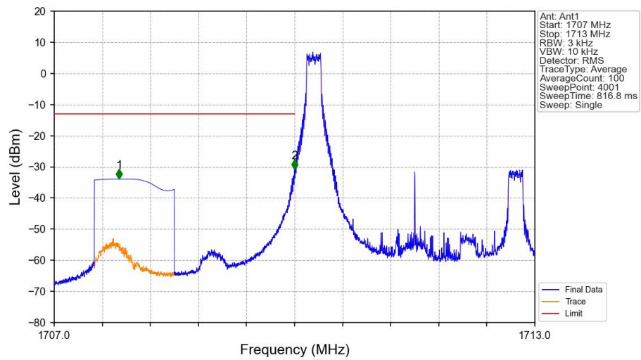
Band4_3MHz_16QAM_LCH_1711.5MHz_RB_1_0_NTNV
