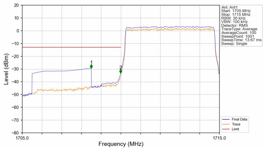
Band4_5MHz_QPSK_LCH_1712.5MHz_RB_25_0_NTNV
