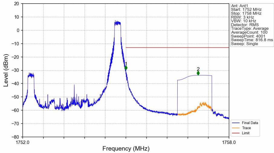
Band4_3MHz_16QAM_HCH_1753.5MHz_RB_1_14_NTNV
