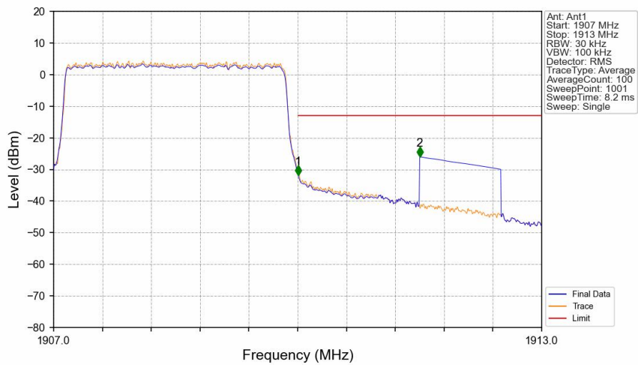
Band2_3MHz_16QAM_HCH_1908.5MHz_RB_15_0_NTNV
