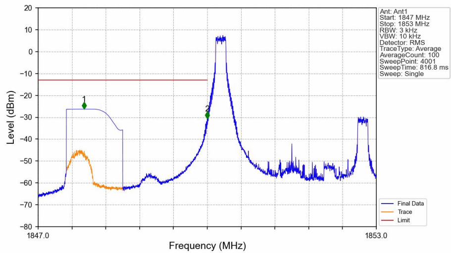
Band2_3MHz_16QAM_LCH_1851.5MHz_RB_1_0_NTNV
