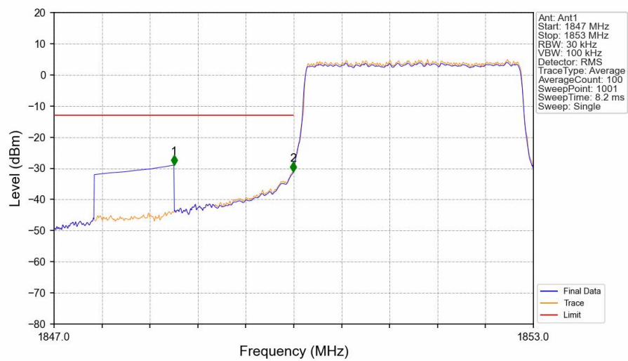
Band2_3MHz_QPSK_LCH_1851.5MHz_RB_15_0_NTNV
