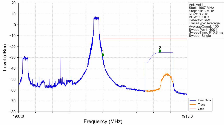
Band2_3MHz_16QAM_HCH_1908.5MHz_RB_1_14_NTNV
