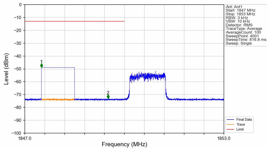
Band2_1.4MHz_16QAM_LCH_1850.7MHz_RB_1_0_NTNV
