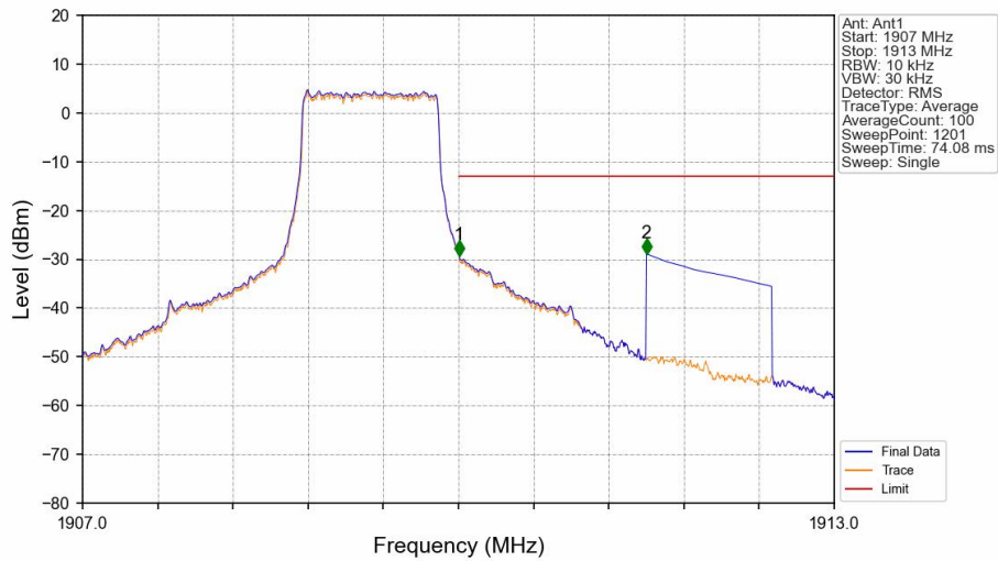
Band2_1.4MHz_QPSK_HCH_1909.3MHz_RB_6_0_NTNV
