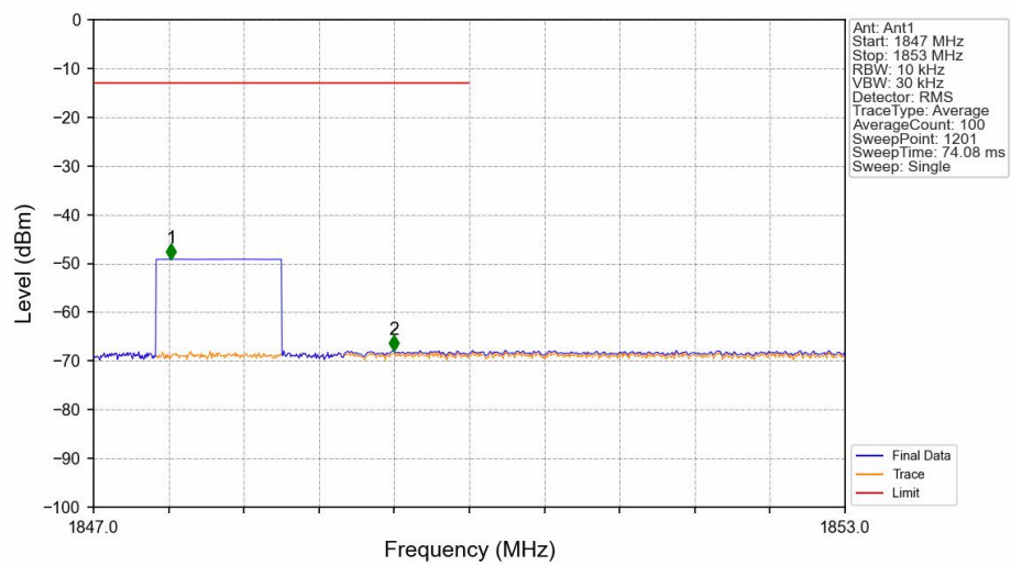
Band2_1.4MHz_QPSK_LCH_1850.7MHz_RB_6_0_NTNV
