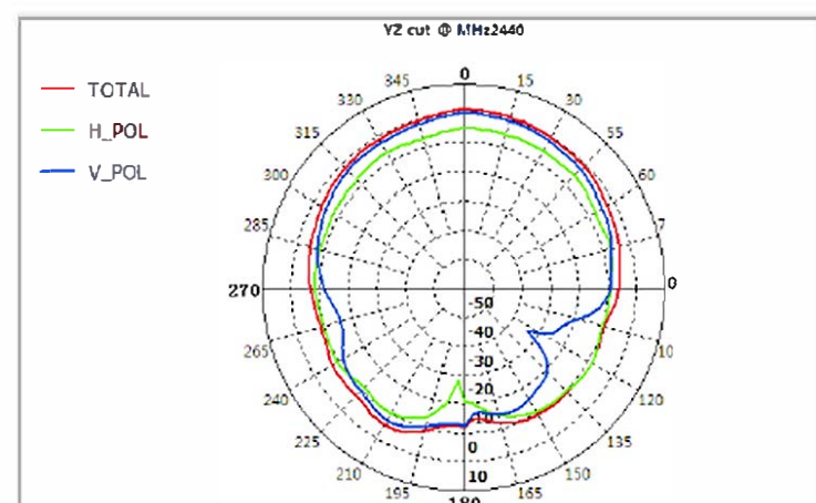
2D-plane YOZ @2.44GHz
