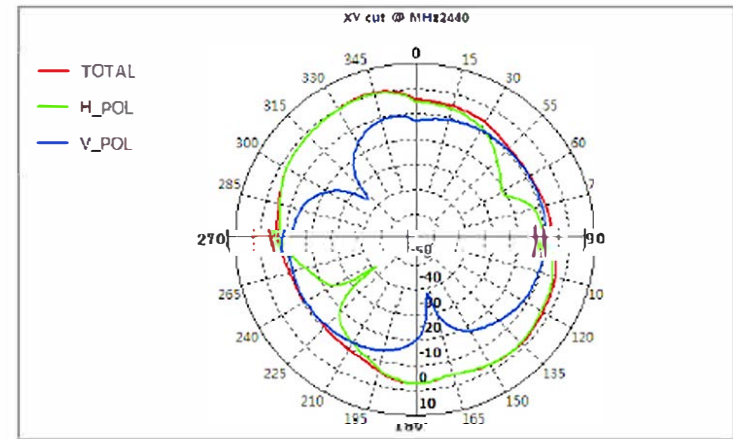
2D-plane XOY @2.44GHz
