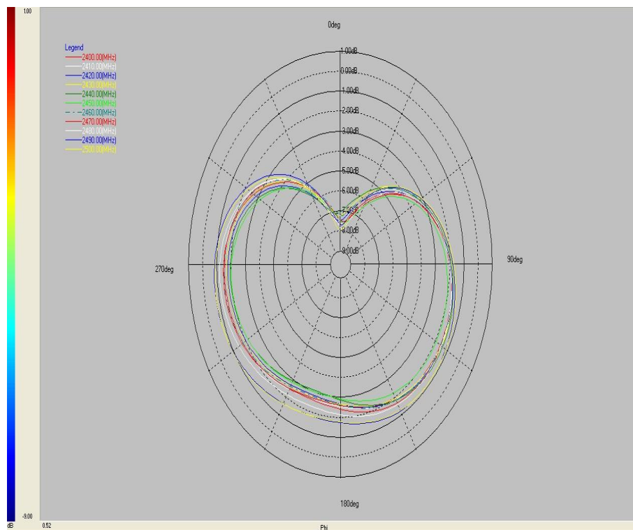
PHI 90 degrees
