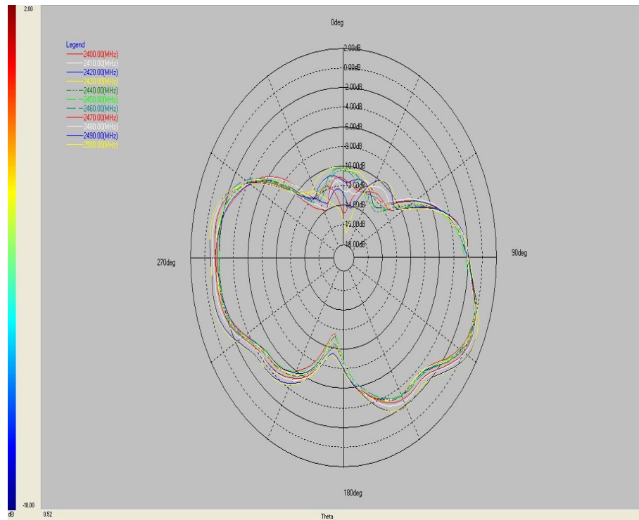
PHI 0 Degree
