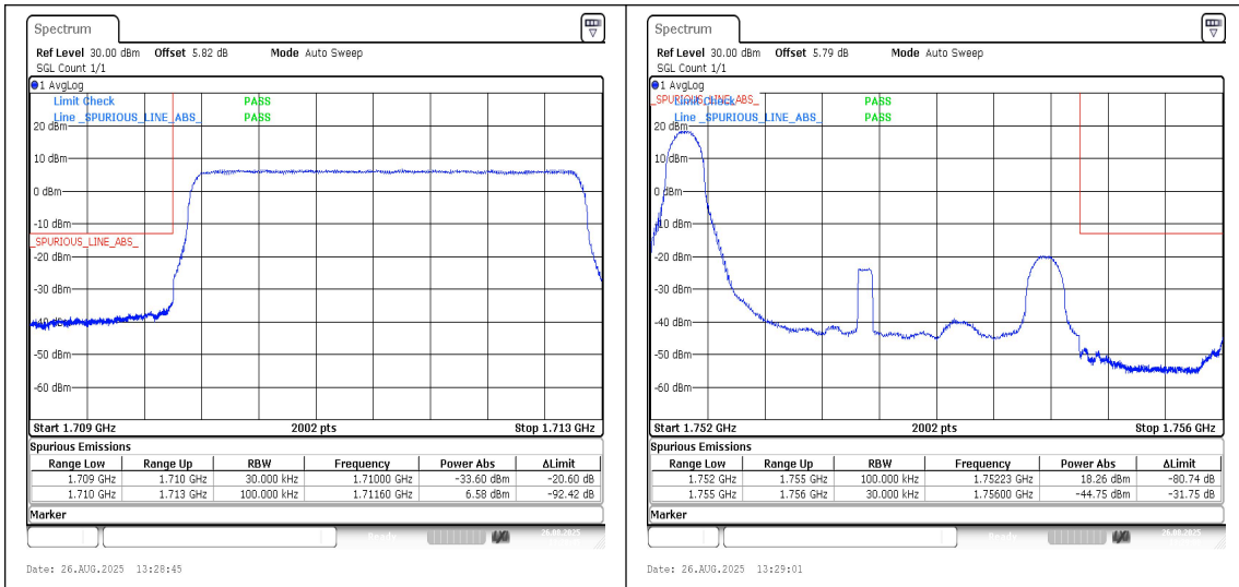
Band4-3MHz-16QAM-19965-15RB#0-PASS Band4-3MHz-QPSK-20385-1RB#0-PASS
