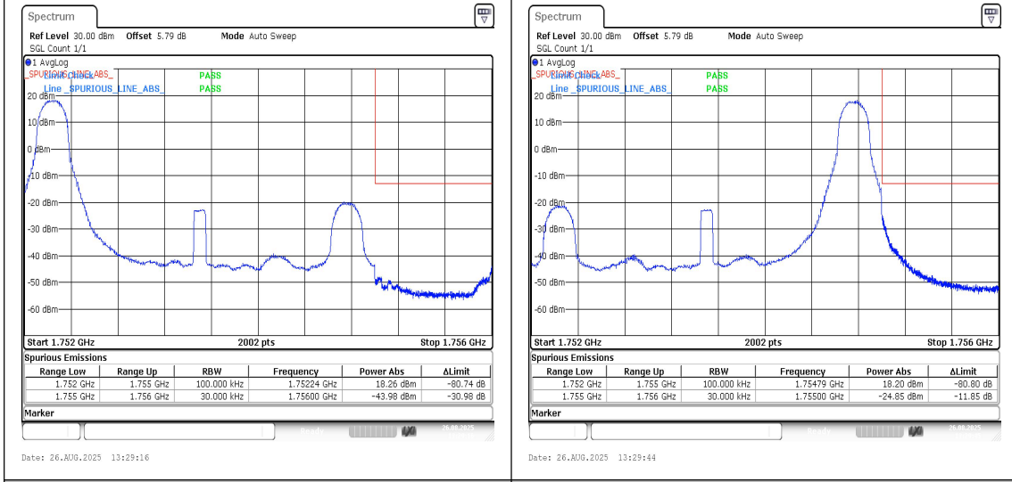
Band4-3MHz-16QAM-20385-1RB#0-PASS Band4-3MHz-16QAM-20385-1RB#14-PASS
