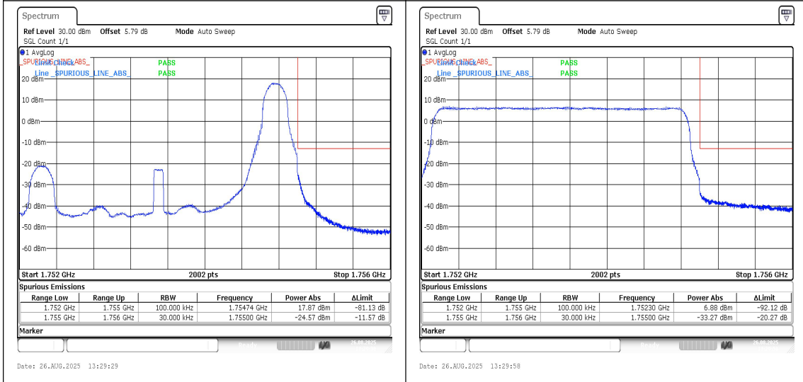
Band4-3MHz-QPSK-20385-1RB#14-PASS Band4-3MHz-QPSK-20385-15RB#0-PASS
