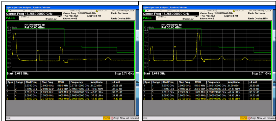
Band41_15MHz_16QAM_41515_1RB#0
