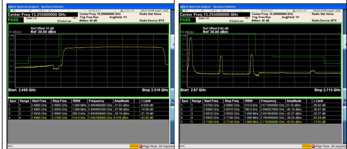
Band41_20MHz_QPSK_39750_100RB#0
