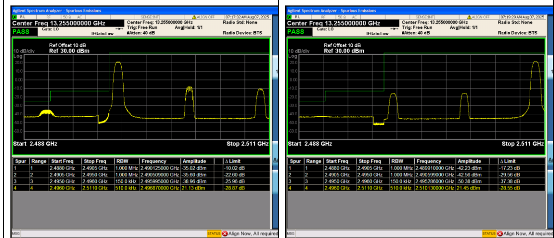
Band41_15MHz_16QAM_39725_1RB#0
