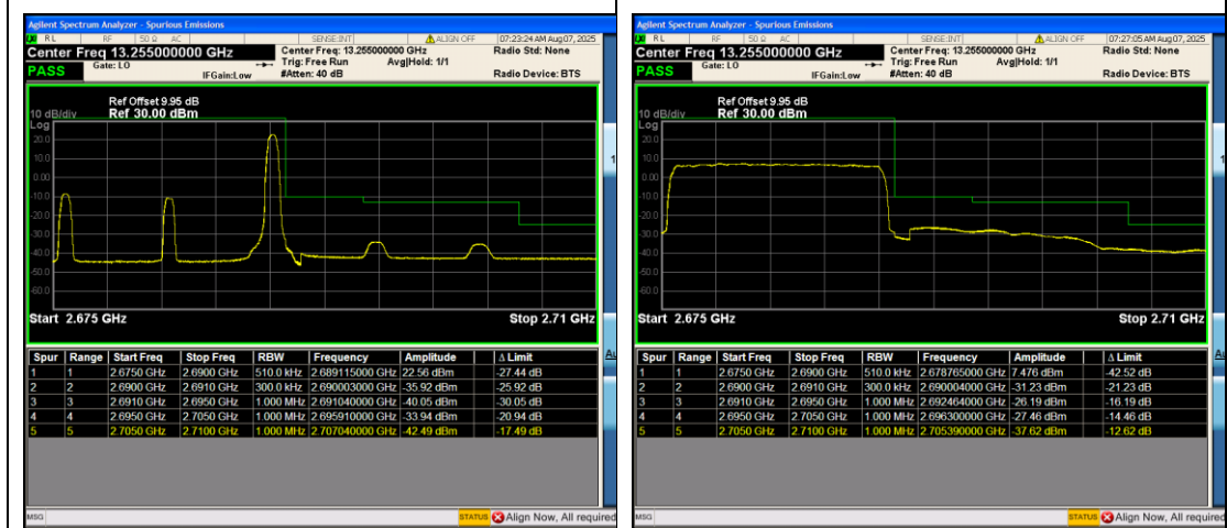
Band41_15MHz_QPSK_41515_1RB#74
