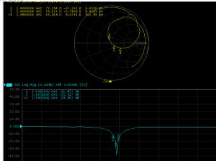
Return Loss
