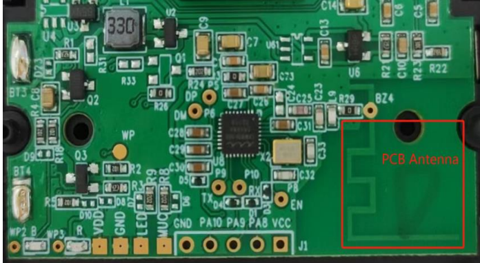
Antenna photo(Unit:mm)
