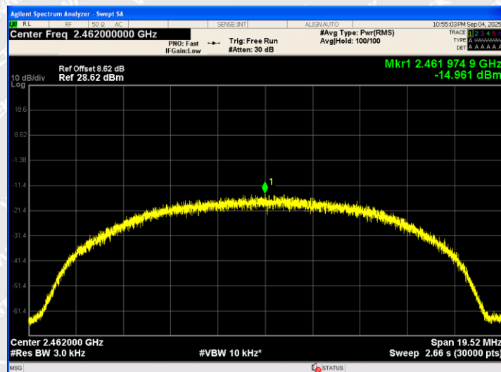
802.11b_High Channel
