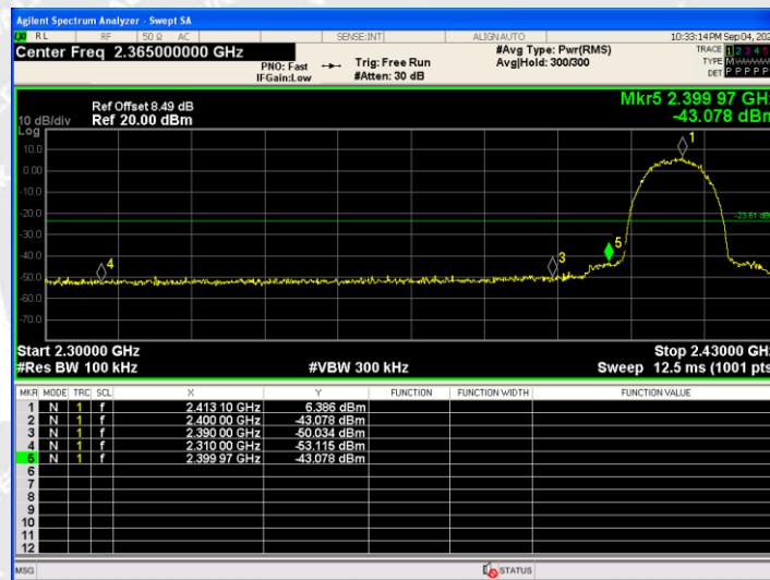
802.11b_Low Channel
