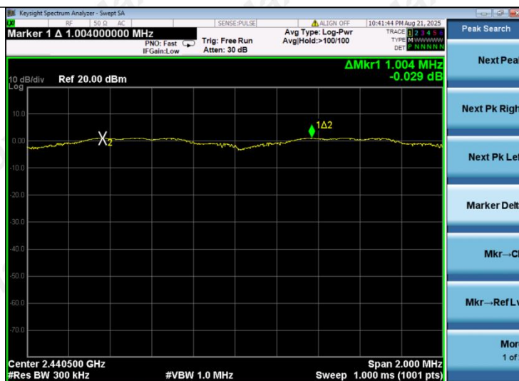
8-DPSK
