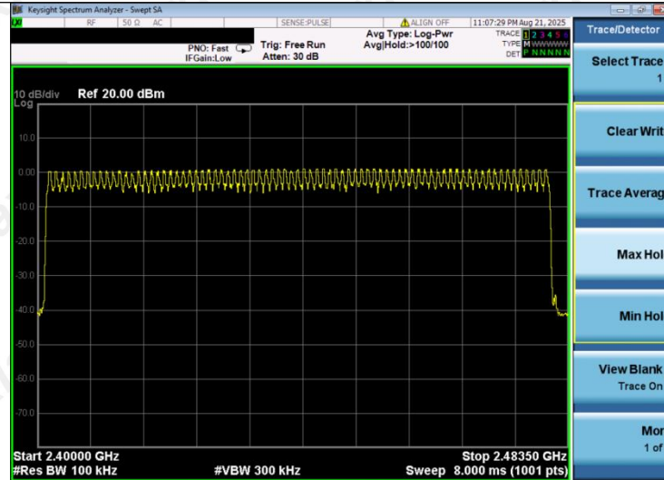
8-DPSK Modulation
