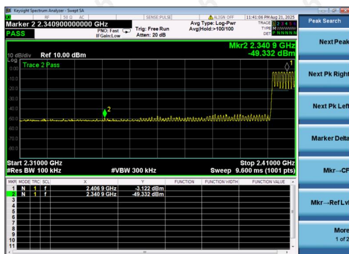
Left Band edge hoping on
