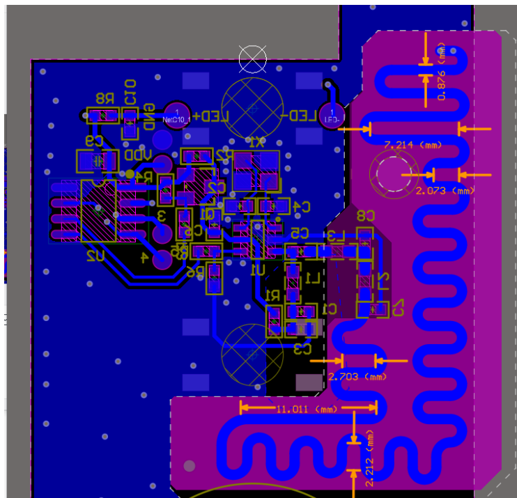
Picture of antenna
