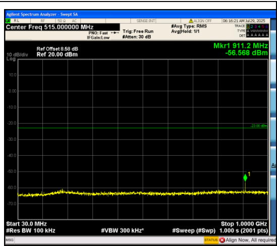
Band66_15MHz_16QAM_132047_75RB#0_30~ 1000_30~1000
