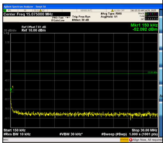
Band66_15MHz_QPSK_132047_75RB#0_0.15~ 30_0.15~30
