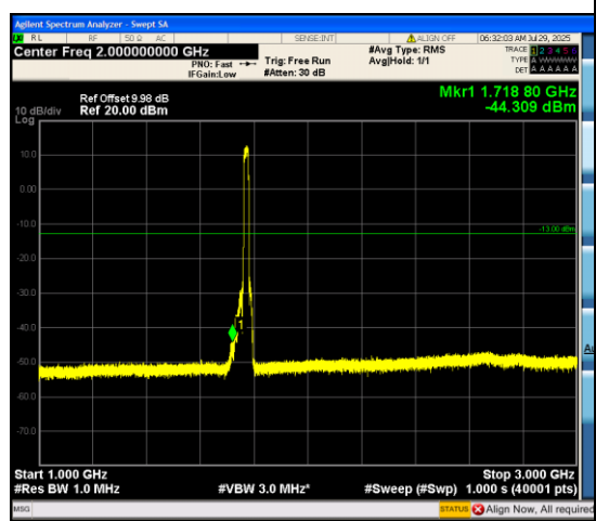
Band66_20MHz_QPSK_132572_100RB#0_100 0~3000_1000~3000
