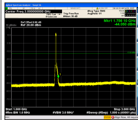
Band66_15MHz_16QAM_132047_75RB#0_100 0~3000_1000~3000
