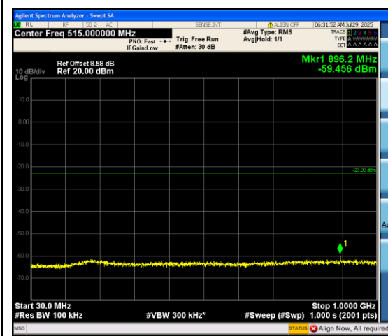
Band66_20MHz_QPSK_132572_100RB#0_30~ 1000_30~1000
