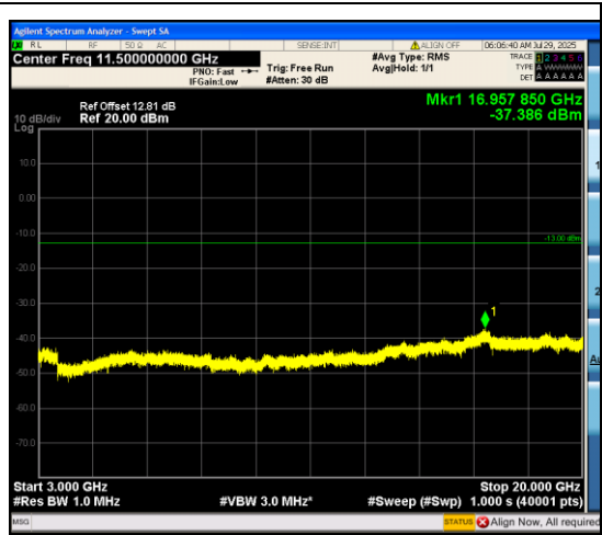
Band66_10MHz_16QAM_132622_50RB#0_300 0~20000_3000~20000
