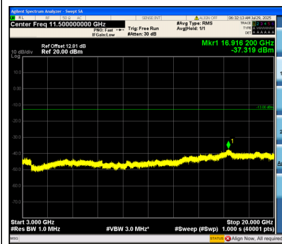
Band66_20MHz_QPSK_132572_100RB#0_300 0~20000_3000~20000
