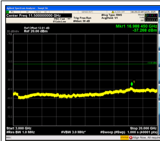
Band66_20MHz_QPSK_132072_100RB#0_300 0~20000_3000~20000
