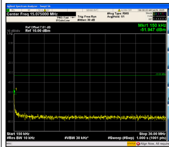
Band66_20MHz_QPSK_132322_100RB#0_0.15 ~30_0.15~30
