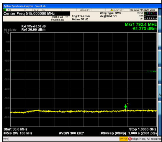
Band66_20MHz_QPSK_132322_100RB#0_30~ 1000_30~1000
