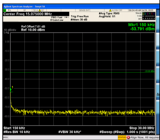
Band66_10MHz_16QAM_132322_50RB#0_0.15 ~30_0.15~30
