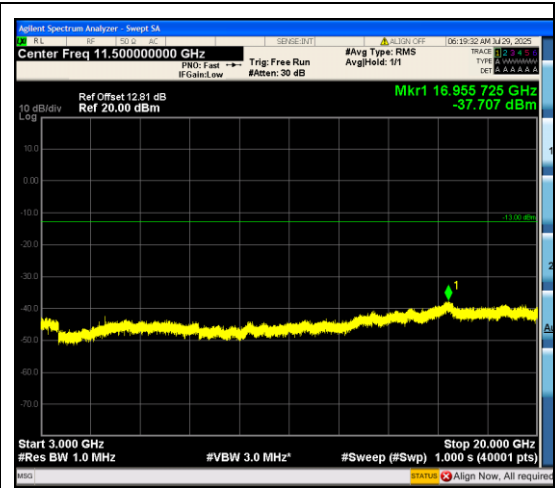
Band66_15MHz_16QAM_132597_75RB#0_300 0~20000_3000~20000
