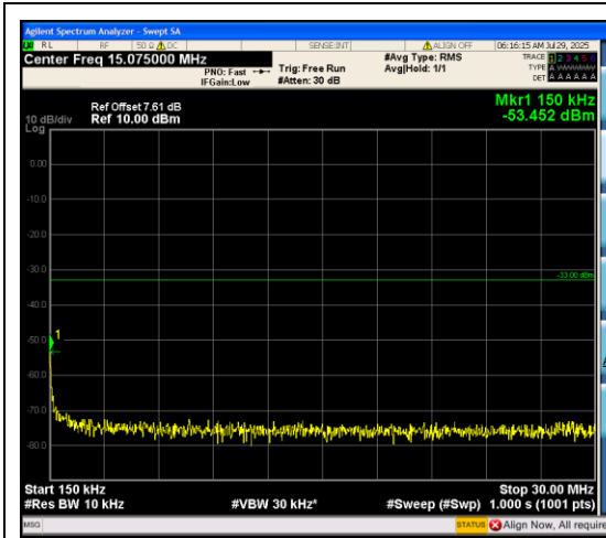
Band66_15MHz_16QAM_132047_75RB#0_0.15 ~30_0.15~30
