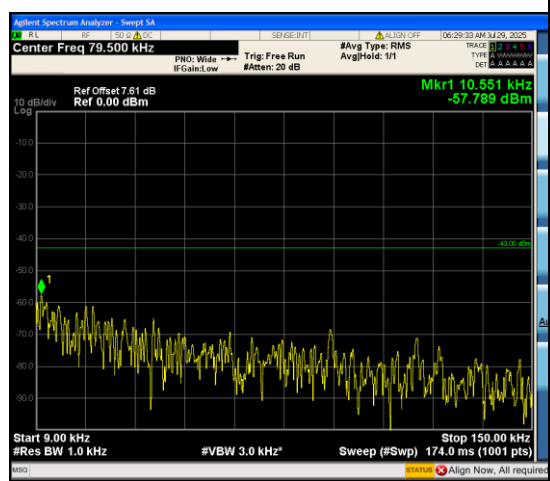
Band66_20MHz_16QAM_132072_100RB#0_0.0 09~0.15_0.009~0.15
