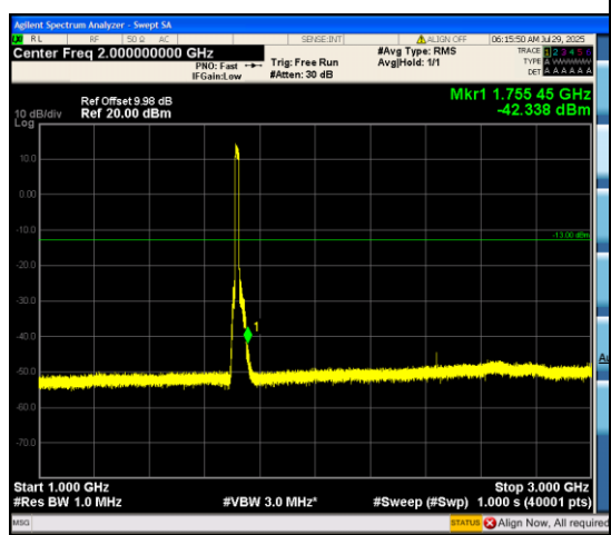
Band66_15MHz_QPSK_132047_75RB#0_1000 ~3000_1000~3000
