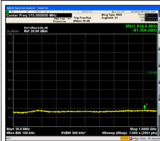
Band66_20MHz_QPSK_132072_100RB#0_30~ 1000_30~1000
