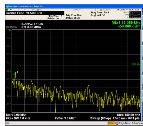
Band66_20MHz_QPSK_132072_100RB#0_0.00 9~0.15_0.009~0.15
