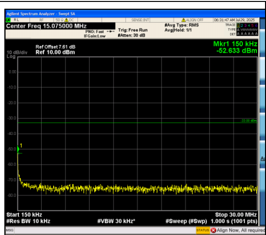
Band66_20MHz_QPSK_132572_100RB#0_0.15 ~30_0.15~30
