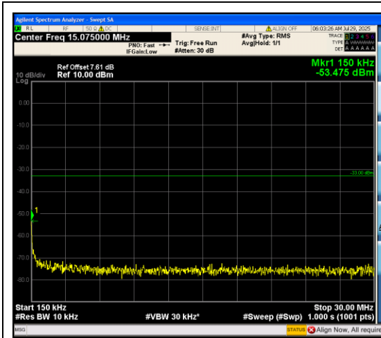
Band66_10MHz_16QAM_132022_50RB#0_0.15 ~30_0.15~30
