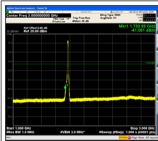
Band66_15MHz_16QAM_132597_75RB#0_100 0~3000_1000~3000
