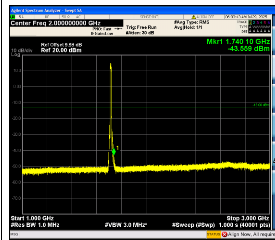
Band66_10MHz_16QAM_132022_50RB#0_100 0~3000_1000~3000
