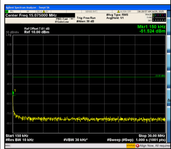
Band66_20MHz_QPSK_132072_100RB#0_0.15 ~30_0.15~30
