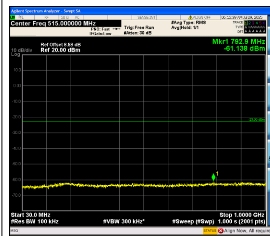
Band66_15MHz_QPSK_132047_75RB#0_30~1 000_30~1000
