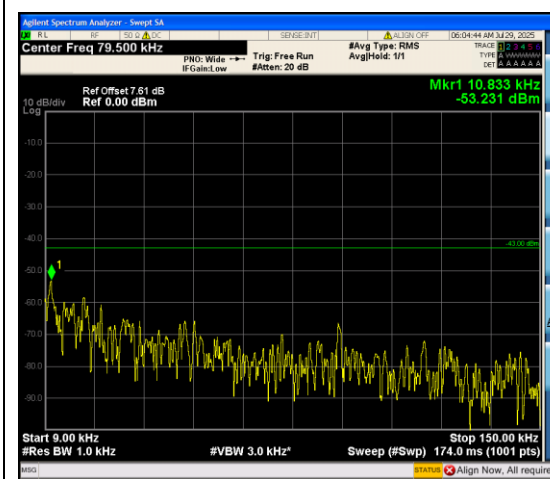
Band66_10MHz_16QAM_132322_50RB#0_0.00 9~0.15_0.009~0.15
