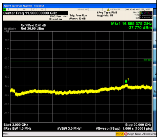
Band66_20MHz_QPSK_132322_100RB#0_300 0~20000_3000~20000
