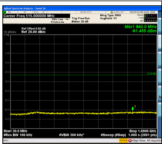
Band66_10MHz_16QAM_132022_50RB#0_30~ 1000_30~1000
