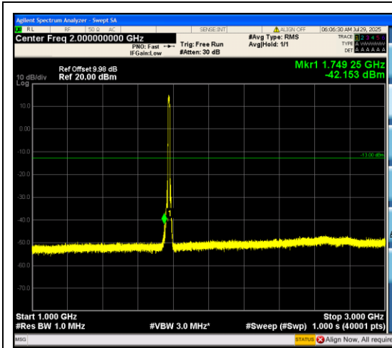
Band66_10MHz_16QAM_132622_50RB#0_100 0~3000_1000~3000
