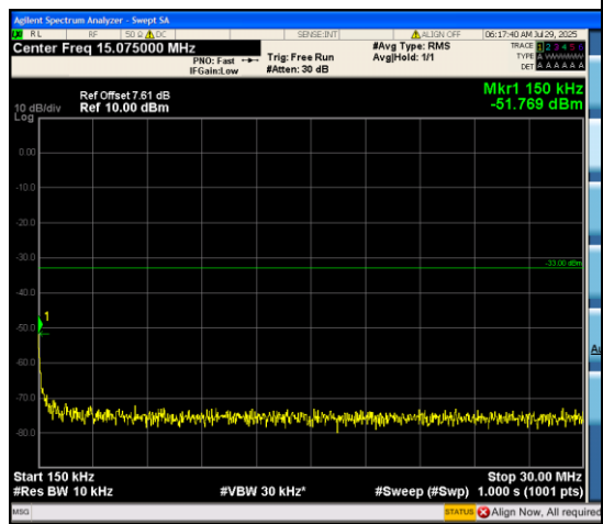
Band66_15MHz_16QAM_132322_75RB#0_0.15 ~30_0.15~30
