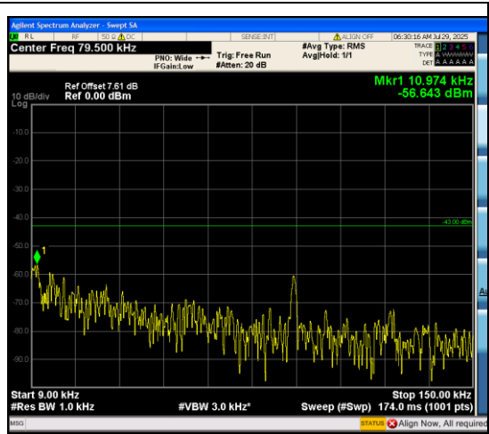
Band66_20MHz_QPSK_132322_100RB#0_0.00 9~0.15_0.009~0.15
