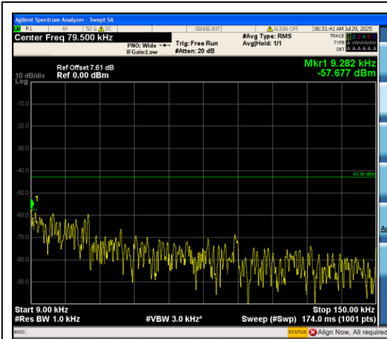
Band66_20MHz_QPSK_132572_100RB#0_0.0 9~0.15_0.009~0.15
