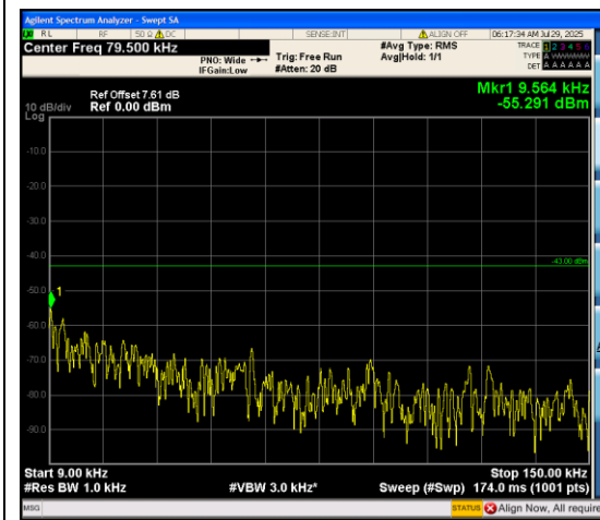
Band66_15MHz_16QAM_132322_75RB#0_0.00 9~0.15_0.009~0.15
