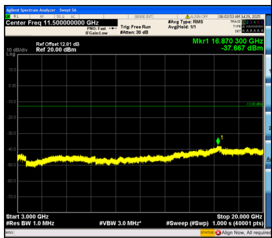
Band66_10MHz_16QAM_132022_50RB#0_300 0~20000_3000~20000
