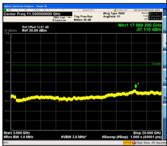
Band66_15MHz_16QAM_132047_75RB#0_300 0~20000_3000~20000
