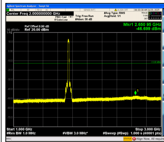
Band66_20MHz_QPSK_132322_100RB#0_100 0~3000_1000~3000
