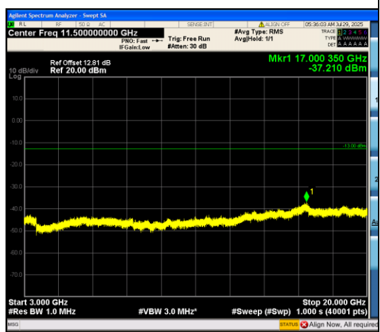
Band66_3MHz_16QAM_131987_15RB#0_3000~20000_3000~20000
