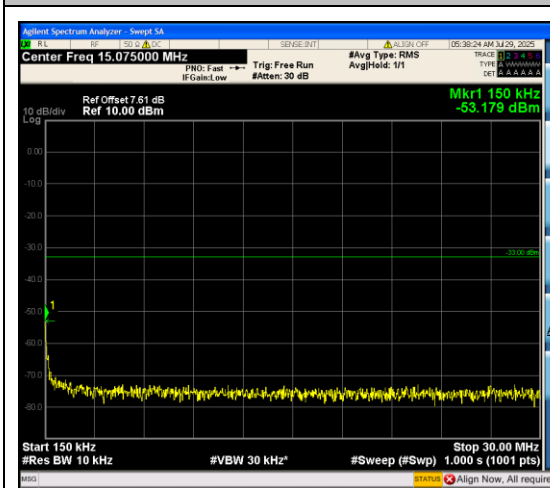
Band66_3MHz_16QAM_132657_15RB#0_0.15~ 30_0.15~30
