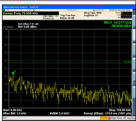
Band66_5MHz_QPSK_132322_25RB#0_0.009~ 0.15_0.009~0.15
