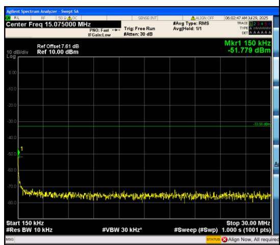
Band66_10MHz_QPSK_132022_50RB#0_0.15~ 30_0.15~30
