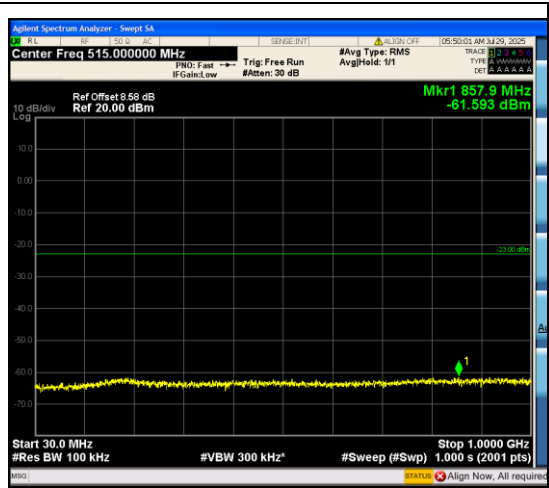
Band66_5MHz_16QAM_131997_25RB#0_30~1 000_30~1000
