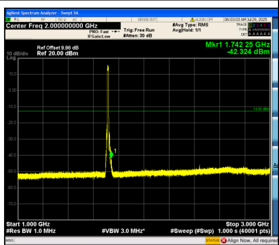
Band66_10MHz_QPSK_132022_50RB#0_1000 ~3000_1000~3000
