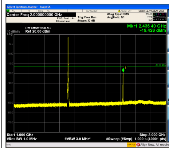
Band66_5MHz_16QAM_131997_25RB#0_1000 ~3000_1000~3000
