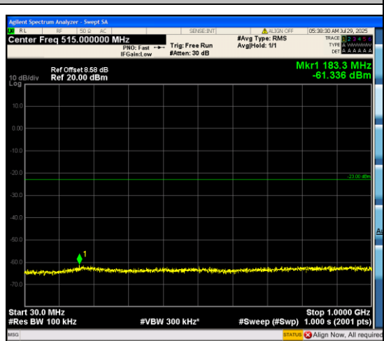
Band66_3MHz_16QAM_132657_15RB#0_30~1 000_30~1000
