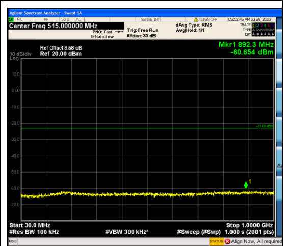
Band66_5MHz_16QAM_132647_25RB#0_30~1 000_30~1000
