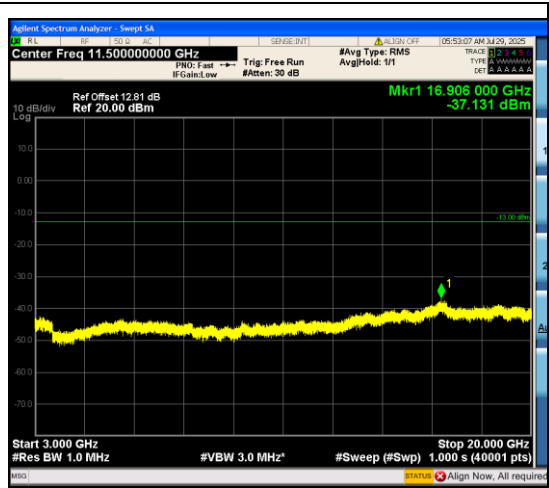
Band66_5MHz_16QAM_132647_25RB#0_3000 ~20000_3000~20000
