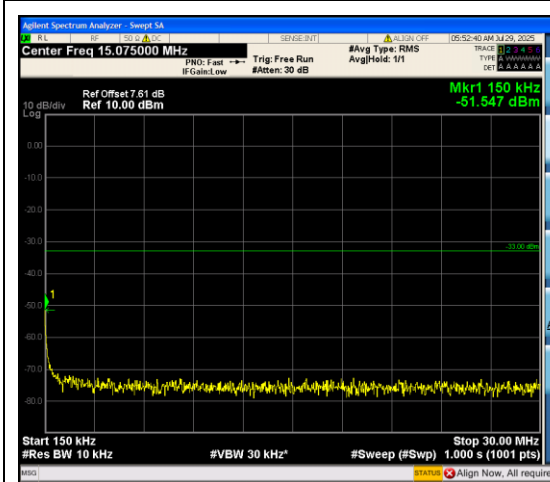
Band66_5MHz_16QAM_132647_25RB#0_0.15~ 30_0.15~30
