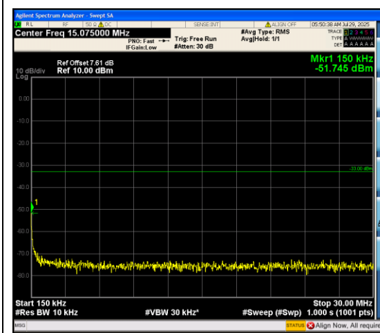
Band66_5MHz_QPSK_132322_25RB#0_0.15~3 0_0.15~30
