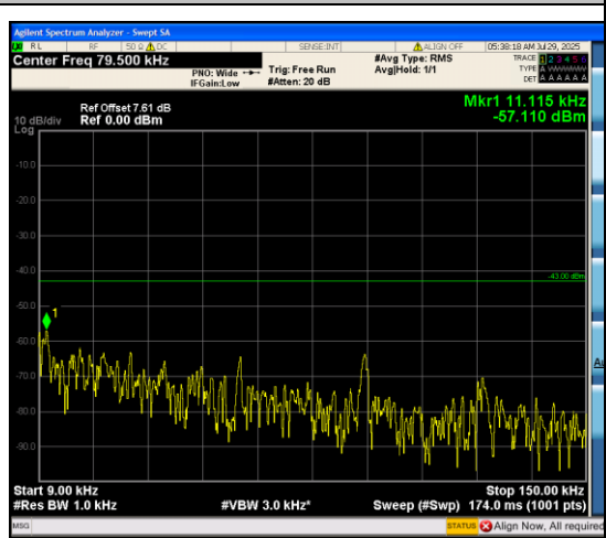
Band66_3MHz_16QAM_132657_15RB#0_0.009 ~0.15_0.009~0.15
