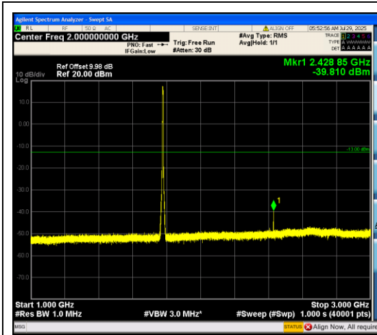
Band66_5MHz_16QAM_132647_25RB#0_1000 ~3000_1000~3000
