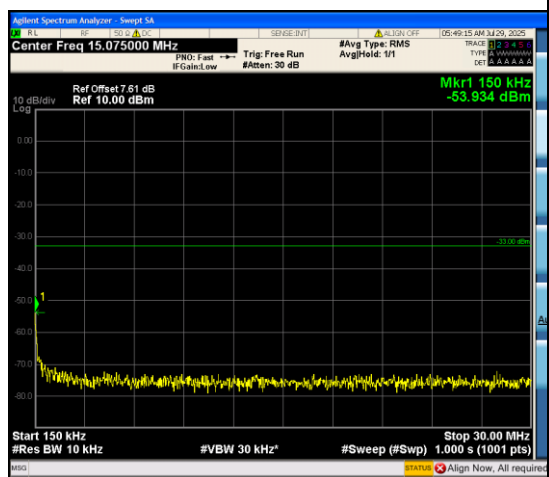
Band66_5MHz_QPSK_131997_25RB#0_0.15~3 0_0.15~30
