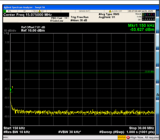
Band66_3MHz_16QAM_132322_15RB#0_0.15~30_0.15~30
