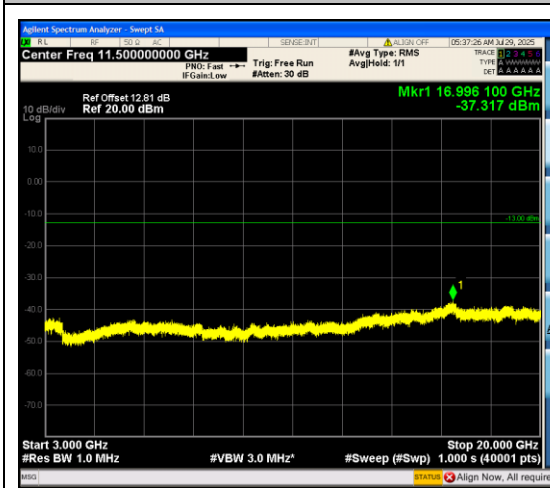
Band66_3MHz_16QAM_132322_15RB#0_3000 ~20000_3000~20000
