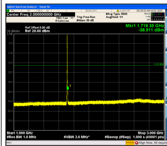
Band66_3MHz_16QAM_131987_15RB#0_1000~3000_1000~3000
