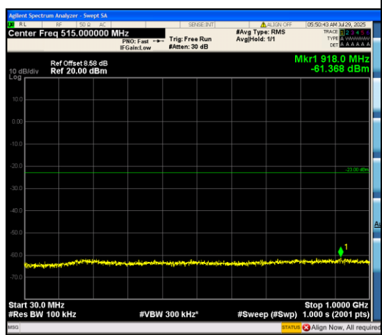
Band66_5MHz_QPSK_132322_25RB#0_30~10 00_30~1000
