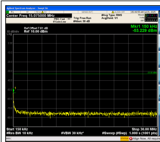
Band66_5MHz_16QAM_131997_25RB#0_0.15~ 30_0.15~30
