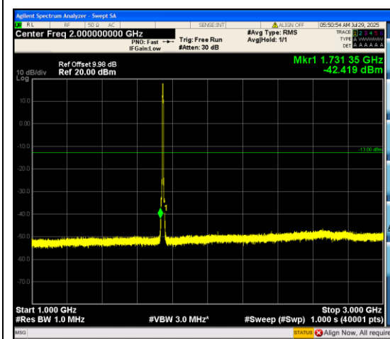
Band66_5MHz_QPSK_132322_25RB#0_1000~ 3000_1000~3000
