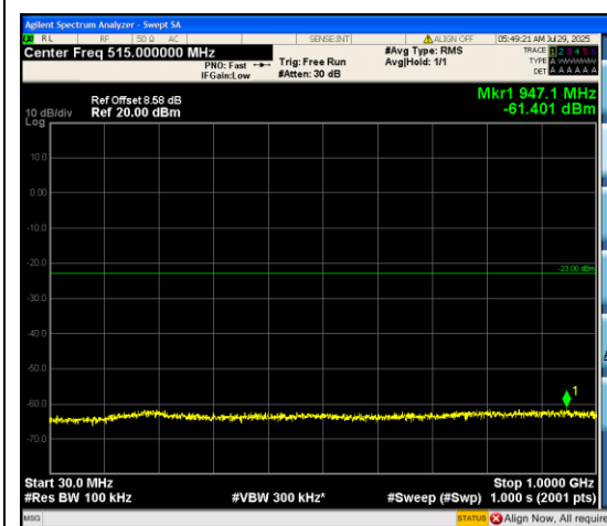
Band66_5MHz_QPSK_131997_25RB#0_30~10 00_30~1000
