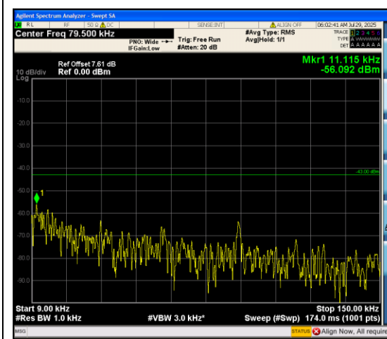
Band66_10MHz_QPSK_132022_50RB#0_0.009 ~0.15_0.009~0.15
