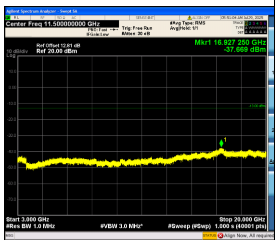
Band66_5MHz_QPSK_132322_25RB#0_3000~ 20000_3000~20000
