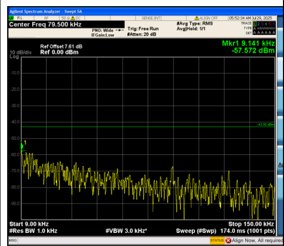
Band66_5MHz_16QAM_132647_25RB#0_0.009 ~0.15_0.009~0.15
