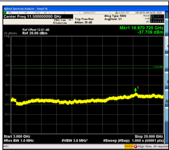
Band66_3MHz_16QAM_132657_15RB#0_3000 ~20000_3000~20000
