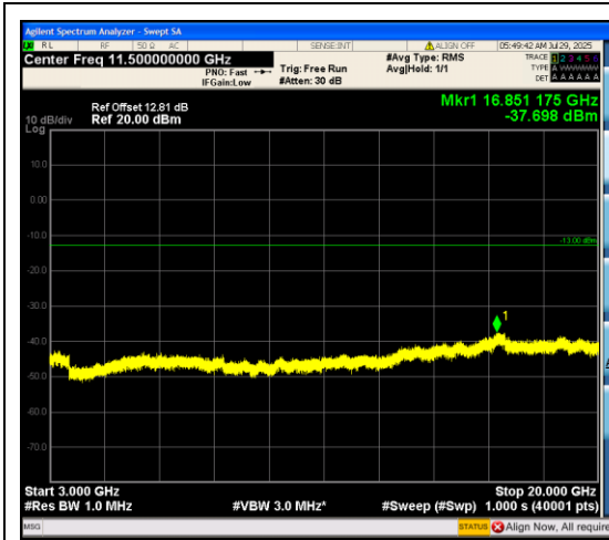
Band66_5MHz_QPSK_131997_25RB#0_3000~ 20000_3000~20000
