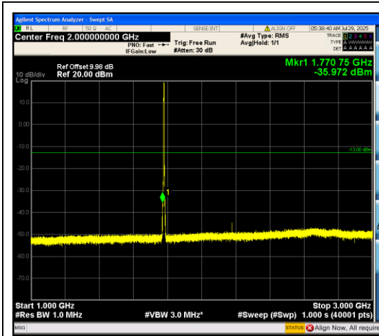
Band66_3MHz_16QAM_132657_15RB#0_1000 ~3000_1000~3000
