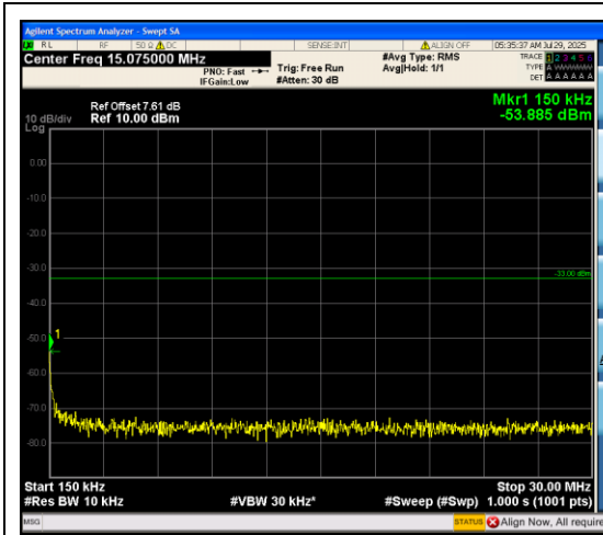
Band66_3MHz_16QAM_131987_15RB#0_0.15~30_0.15~30
