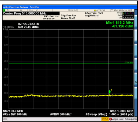
Band66_3MHz_16QAM_131987_15RB#0_30~1000_30~1000
