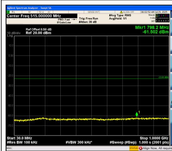
Band66_10MHz_QPSK_132022_50RB#0_30~1 000_30~1000
