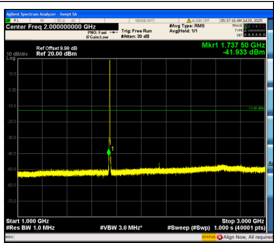
Band66_3MHz_16QAM_132322_15RB#0_1000 ~3000_1000~3000
