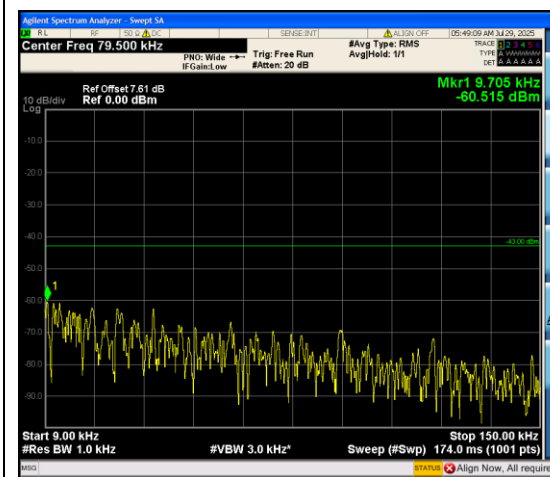
Band66_5MHz_QPSK_131997_25RB#0_0.009~ 0.15_0.009~0.15
