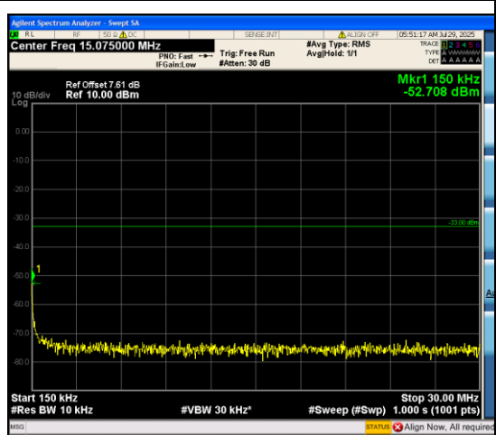
Band66_5MHz_16QAM_132322_25RB#0_0.15~ 30_0.15~30
