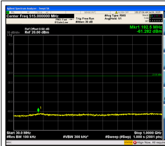
Band66_3MHz_16QAM_132322_15RB#0_30~1 000_30~1000
