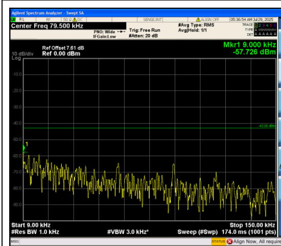
Band66_3MHz_16QAM_132322_15RB#0_0.009~0.15_0.009~0.15
