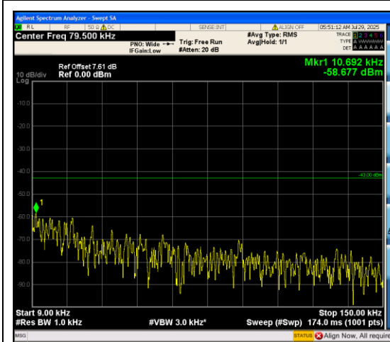
Band66_5MHz_16QAM_132322_25RB#0_0.009 ~0.15_0.009~0.15
