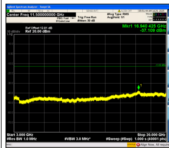
Band66_5MHz_16QAM_132322_25RB#0_3000 ~20000_3000~20000
