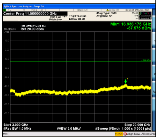
Band66_5MHz_16QAM_131997_25RB#0_3000 ~20000_3000~20000
