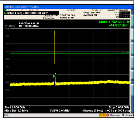
Band66_5MHz_16QAM_132322_25RB#0_1000 ~3000_1000~3000
