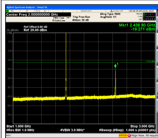
Band66_3MHz_QPSK_132322_15RB#0_1000~ 3000_1000~3000
