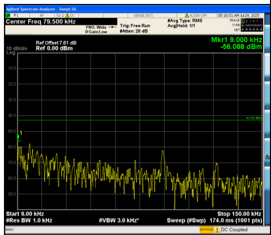
Band66_1.4MHz_16QAM_131979_6RB#0_0.00 9~0.15_0.009~0.15
