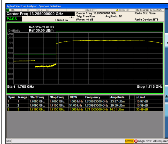
Band66_5MHz_QPSK_131997_25RB#0
