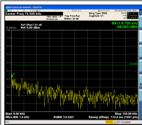
Band66_1.4MHz_QPSK_132665_6RB#0_0.009 ~0.15_0.009~0.15
