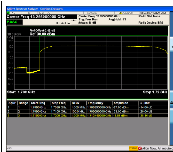
Band66_10MHz_QPSK_132022_50RB#0
