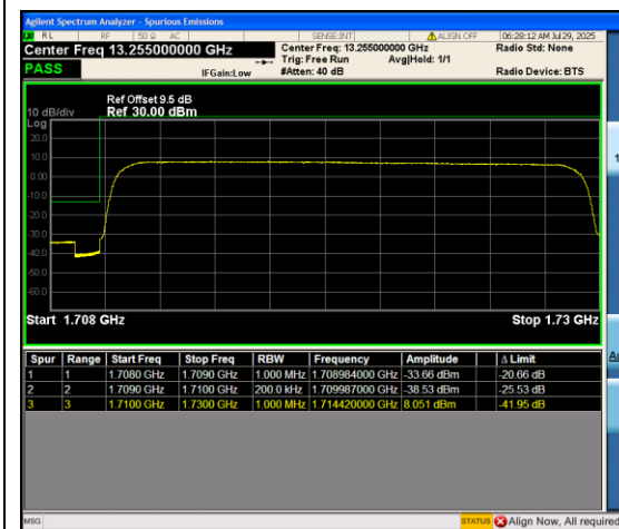
Band66_20MHz_16QAM_132072_100RB#0
