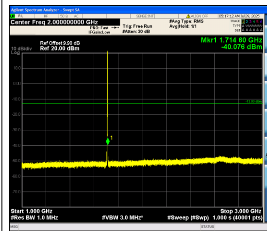
Band66_1.4MHz_16QAM_131979_6RB#0_1000 ~3000_1000~3000
