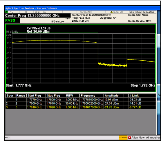
Band66_3MHz_16QAM_132657_15RB#0
