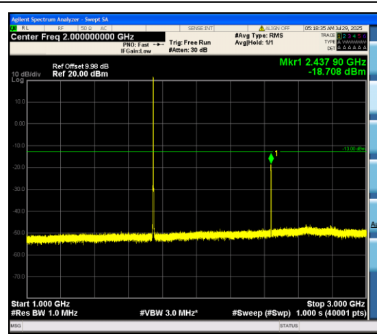
Band66_1.4MHz_16QAM_132322_6RB#0_1000 ~3000_1000~3000
