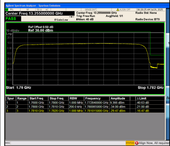
Band66_20MHz_QPSK_132572_100RB#0
