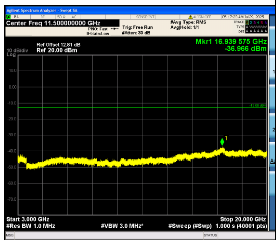
Band66_1.4MHz_16QAM_131979_6RB#0_3000 ~20000_3000~20000
