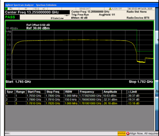
Band66_15MHz_QPSK_132597_75RB#0
