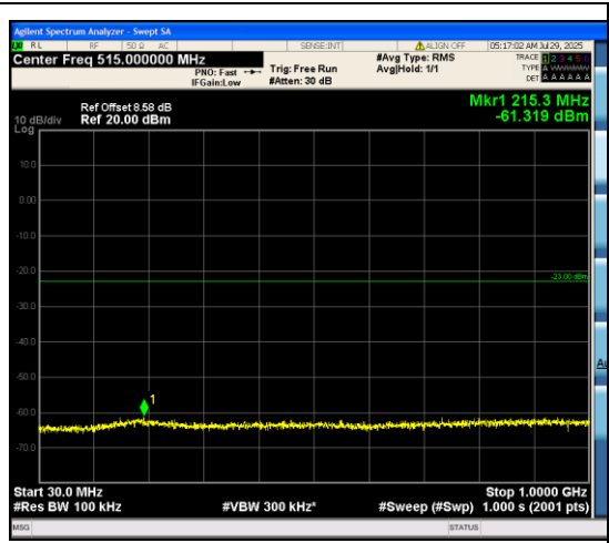
Band66_1.4MHz_16QAM_131979_6RB#0_30~1 000_30~1000
