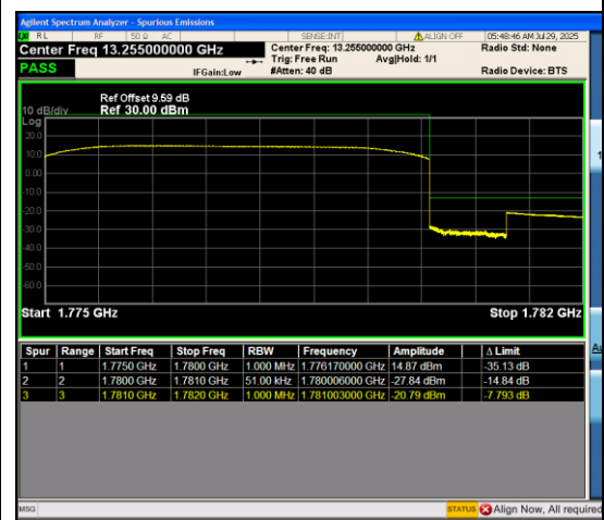
Band66_5MHz_QPSK_132647_25RB#0
