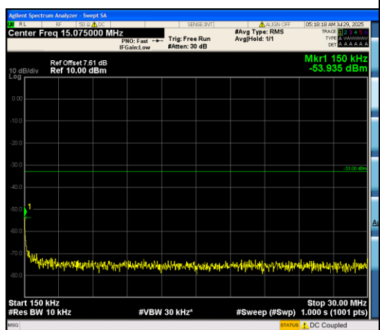
Band66_1.4MHz_16QAM_132322_6RB#0_0.15 ~30_0.15~30
