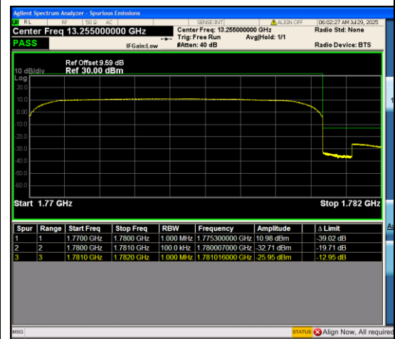
Band66_10MHz_16QAM_132622_50RB#0
