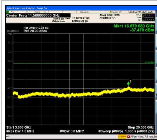
Band66_3MHz_QPSK_131987_15RB#0_3000~ 20000_3000~20000
