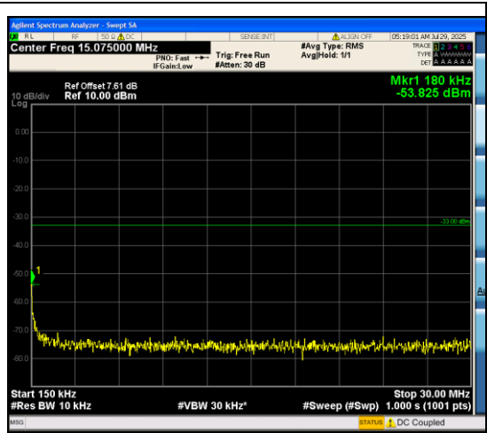
Band66_1.4MHz_QPSK_132665_6RB#0_0.15~ 30_0.15~30
