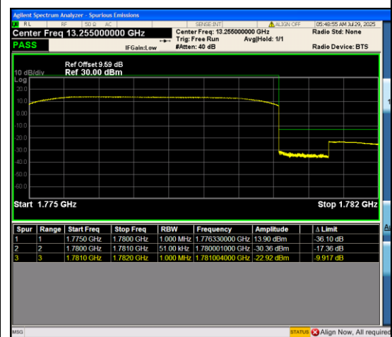
Band66_5MHz_16QAM_132647_25RB#0
