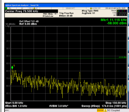
Band66_1.4MHz_16QAM_132322_6RB#0_0.00 9~0.15_0.009~0.15
