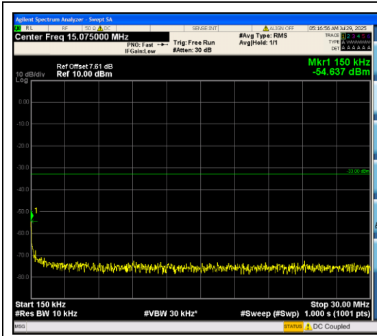
Band66_1.4MHz_16QAM_131979_6RB#0_0.15 ~30_0.15~30
