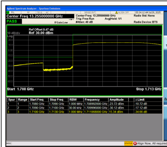
Band66_3MHz_16QAM_131987_15RB#0
