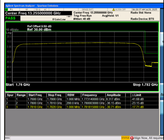
Band66_20MHz_16QAM_132572_100RB#0
