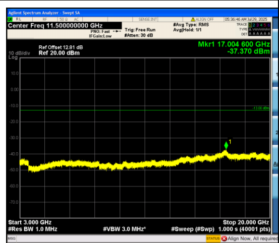
Band66_3MHz_QPSK_132322_15RB#0_3000~ 20000_3000~20000
