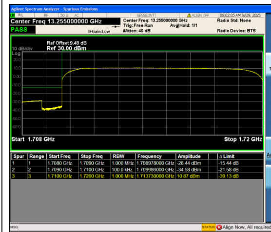
Band66_10MHz_16QAM_132022_50RB#0
