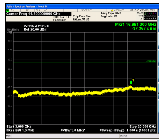
Band66_1.4MHz_16QAM_132322_6RB#0_3000 ~20000_3000~20000
