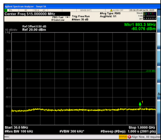
Band66_3MHz_QPSK_132322_15RB#0_30~10 00_30~1000
