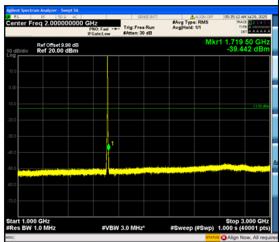
Band66_3MHz_QPSK_131987_15RB#0_1000~ 3000_1000~3000
