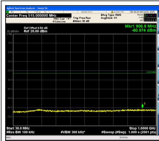
Band66_1.4MHz_16QAM_132322_6RB#0_30~1 000_30~1000
