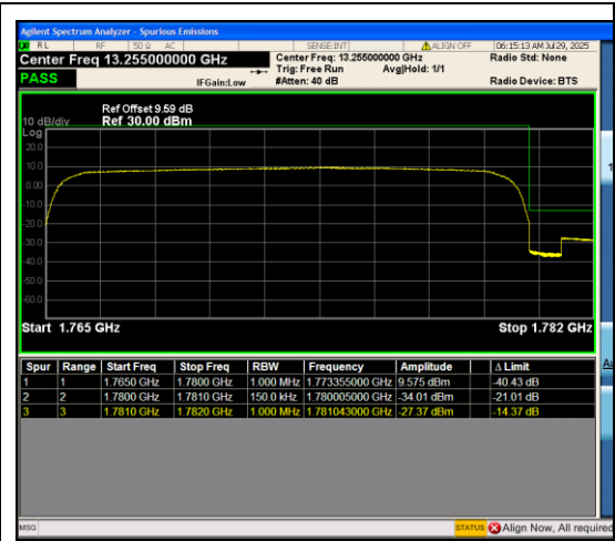
Band66_15MHz_16QAM_132597_75RB#0
