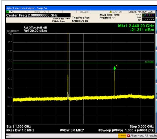
Band66_1.4MHz_16QAM_132665_6RB#0_1000 ~3000_1000~3000
