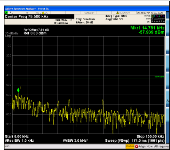
Band66_3MHz_QPSK_132322_15RB#0_0.009~ 0.15_0.009~0.15
