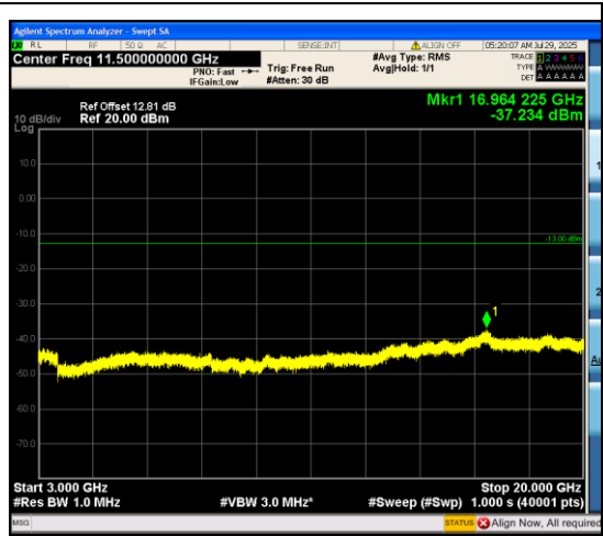
Band66_1.4MHz_16QAM_132665_6RB#0_3000 ~20000_3000~20000
