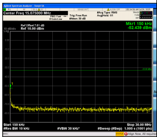
Band66_3MHz_QPSK_131987_15RB#0_0.15~3 0_0.15~30
