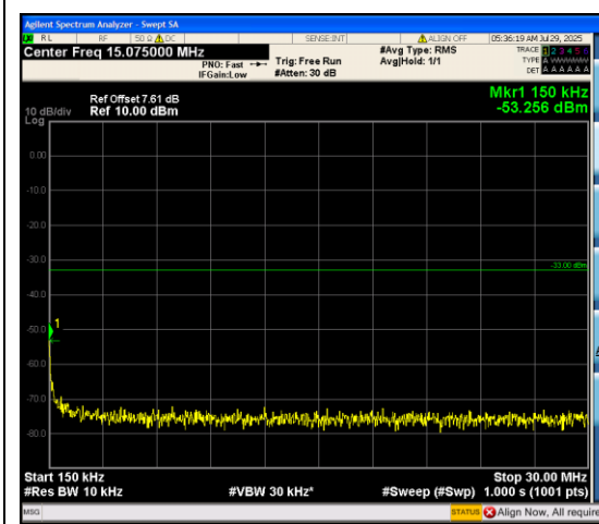
Band66_3MHz_QPSK_132322_15RB#0_0.15~3 0_0.15~30
