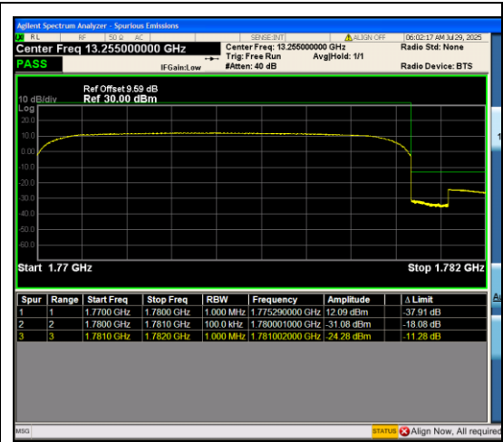
Band66_10MHz_QPSK_132622_50RB#0
