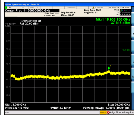
Band66_1.4MHz_QPSK_132665_6RB#0_3000~ 20000_3000~20000
