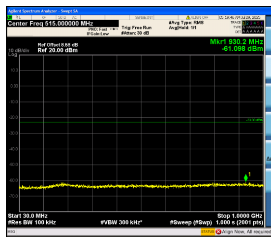
Band66_1.4MHz_16QAM_132665_6RB#0_30~1 000_30~1000
