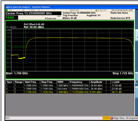
Band66_15MHz_16QAM_132047_75RB#0
