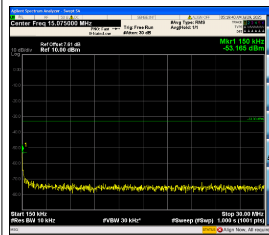
Band66_1.4MHz_16QAM_132665_6RB#0_0.15 ~30_0.15~30
