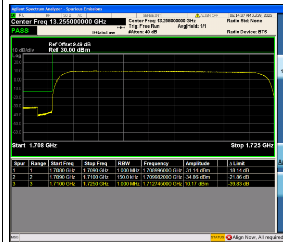
Band66_15MHz_QPSK_132047_75RB#0
