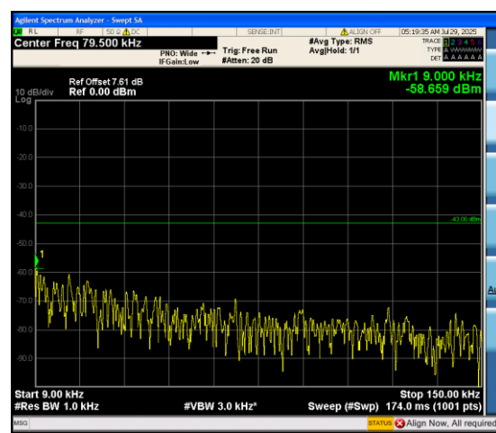
Band66_1.4MHz_16QAM_132665_6RB#0_0.00 9~0.15_0.009~0.15
