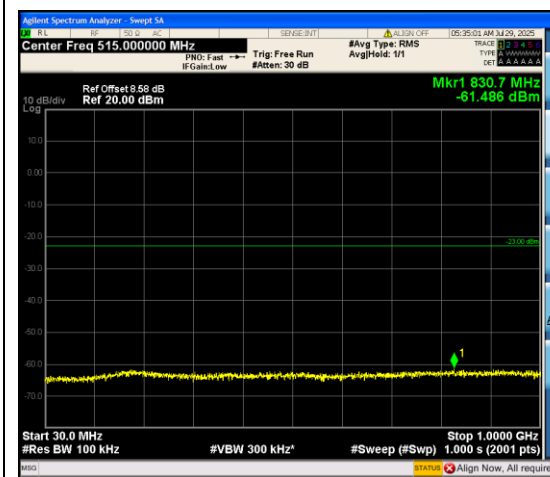
Band66_3MHz_QPSK_131987_15RB#0_30~10 00_30~1000
