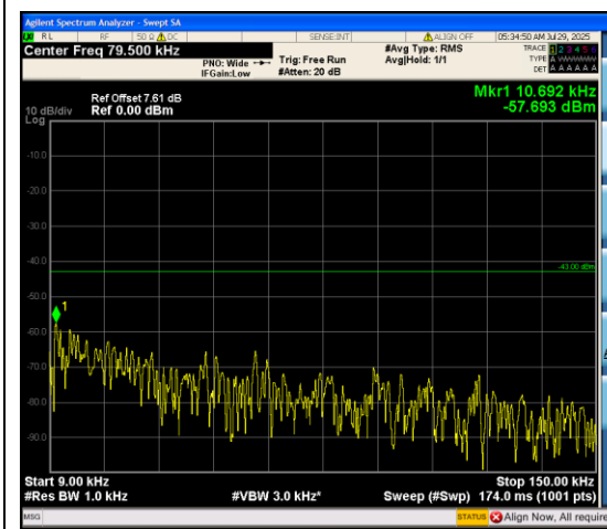
Band66_3MHz_QPSK_131987_15RB#0_0.009~ 0.15_0.009~0.15
