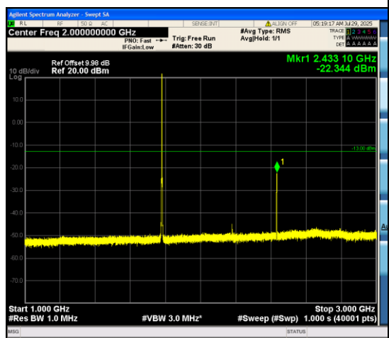
Band66_1.4MHz_QPSK_132665_6RB#0_1000~ 3000_1000~3000
