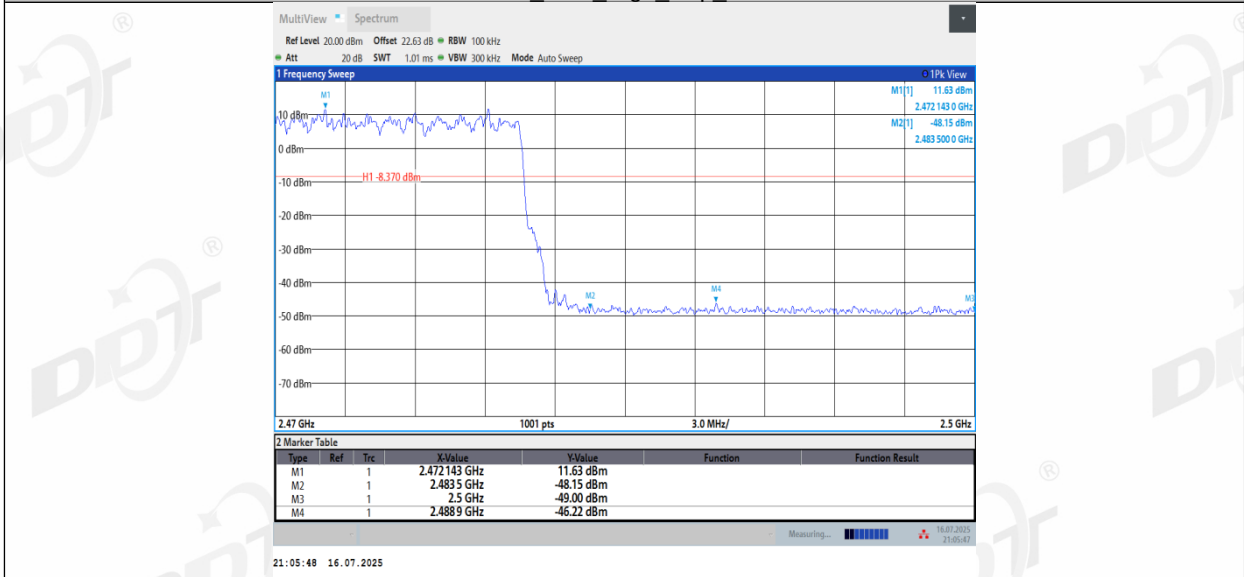
3DH5_Ant2_High_Hop_2480
