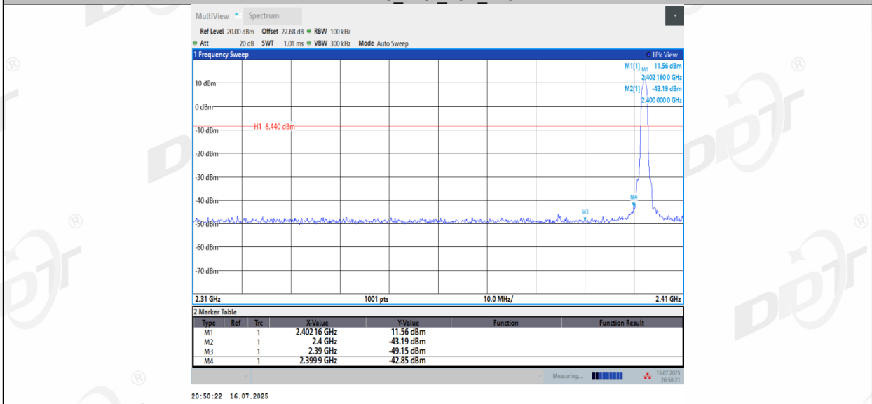
2DH5_Ant2_Low_2402
