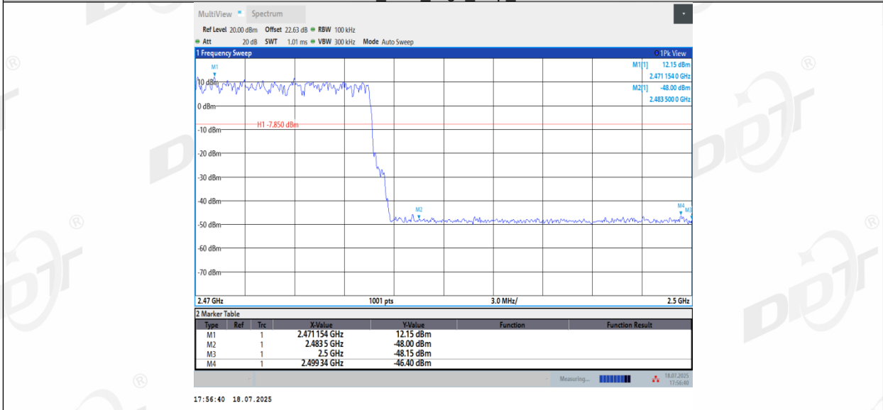
3DH5_Ant2_High_Hop_2480
