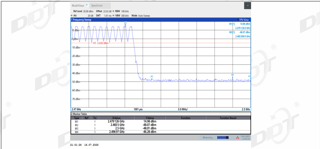
DH5_Ant2_High_Hop_2480
