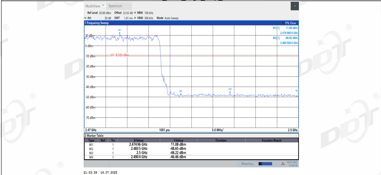
2DH5_Ant2_High_Hop_2480
