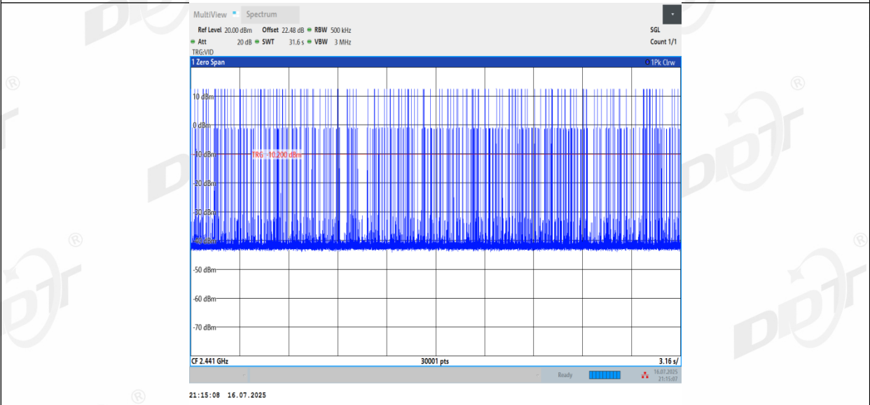
3DH3_Ant2_Hop
