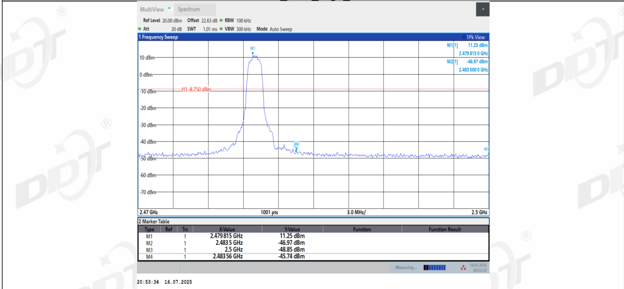
2DH5_Ant2_High_2480
