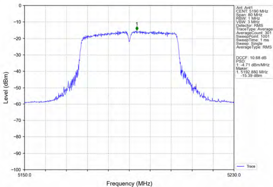
802.11ac(VHT40)_LCH_5190MHz_Ant1_NTNV
