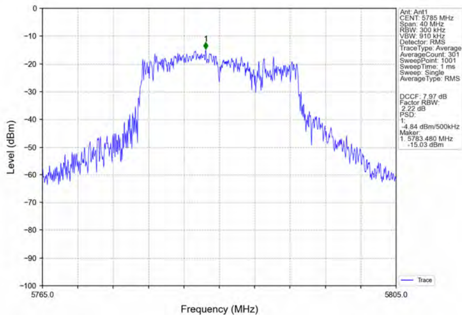
802.11ac(VHT20)_MCH_5785MHz_Ant1_NTNV
