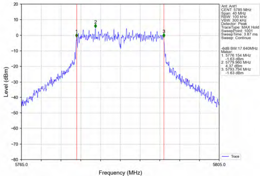
802.11ac(VHT20)_MCH_5785MHz_Ant1_NTNV
