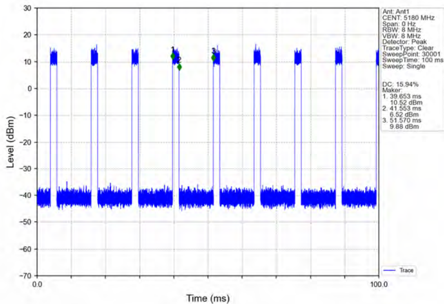
802.11ac(VHT20)_LCH_5180MHz_Ant1_NTNV
