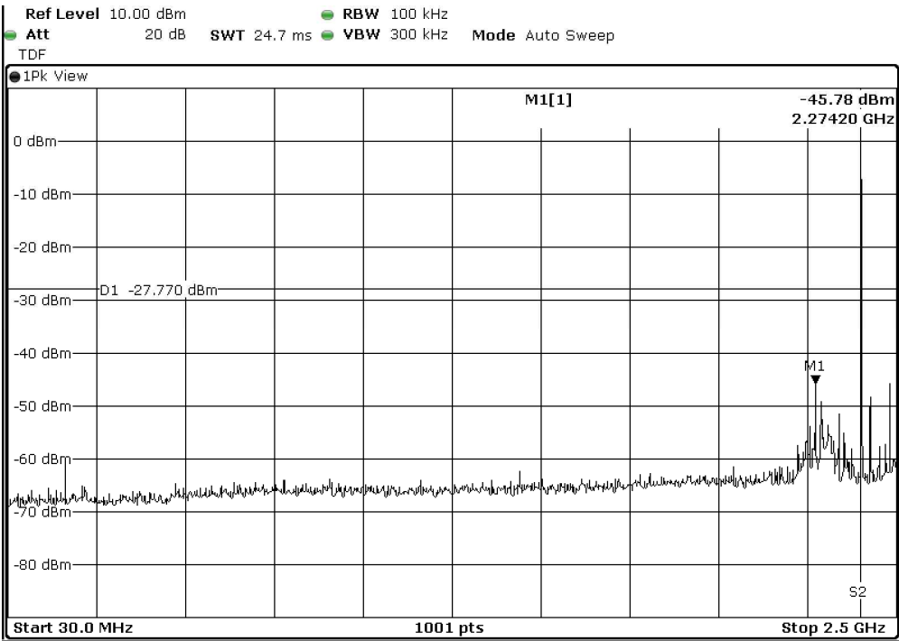
7.1 100 kHz Bandwidth
