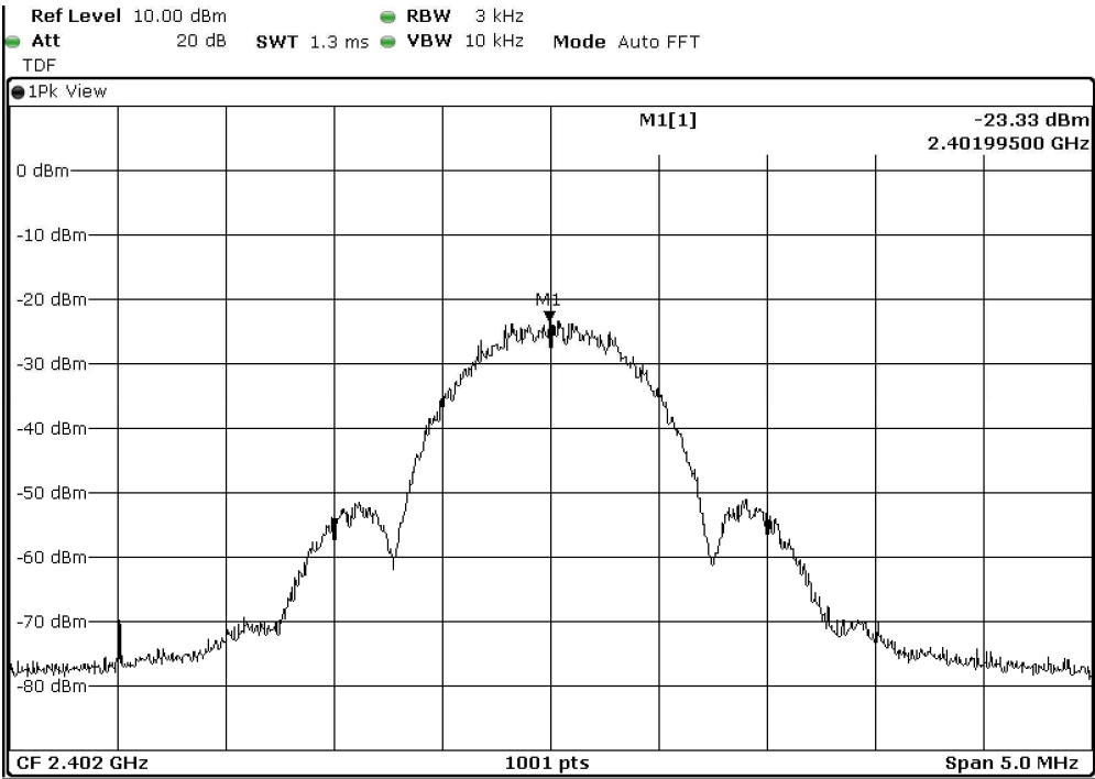
10 Power Spectral Density
