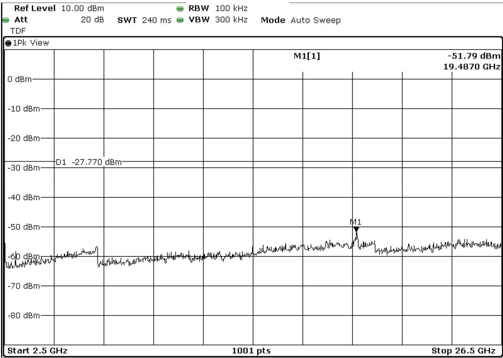
7.2 100 kHz Bandwidth
