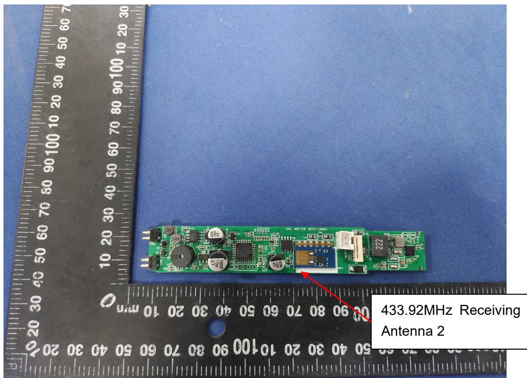
Fig.4 Antenna 2 is only receiving function(433.92MHz)
