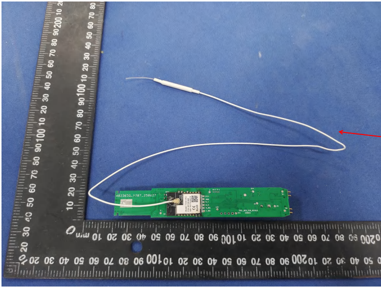
Zigbee Antenna 1
