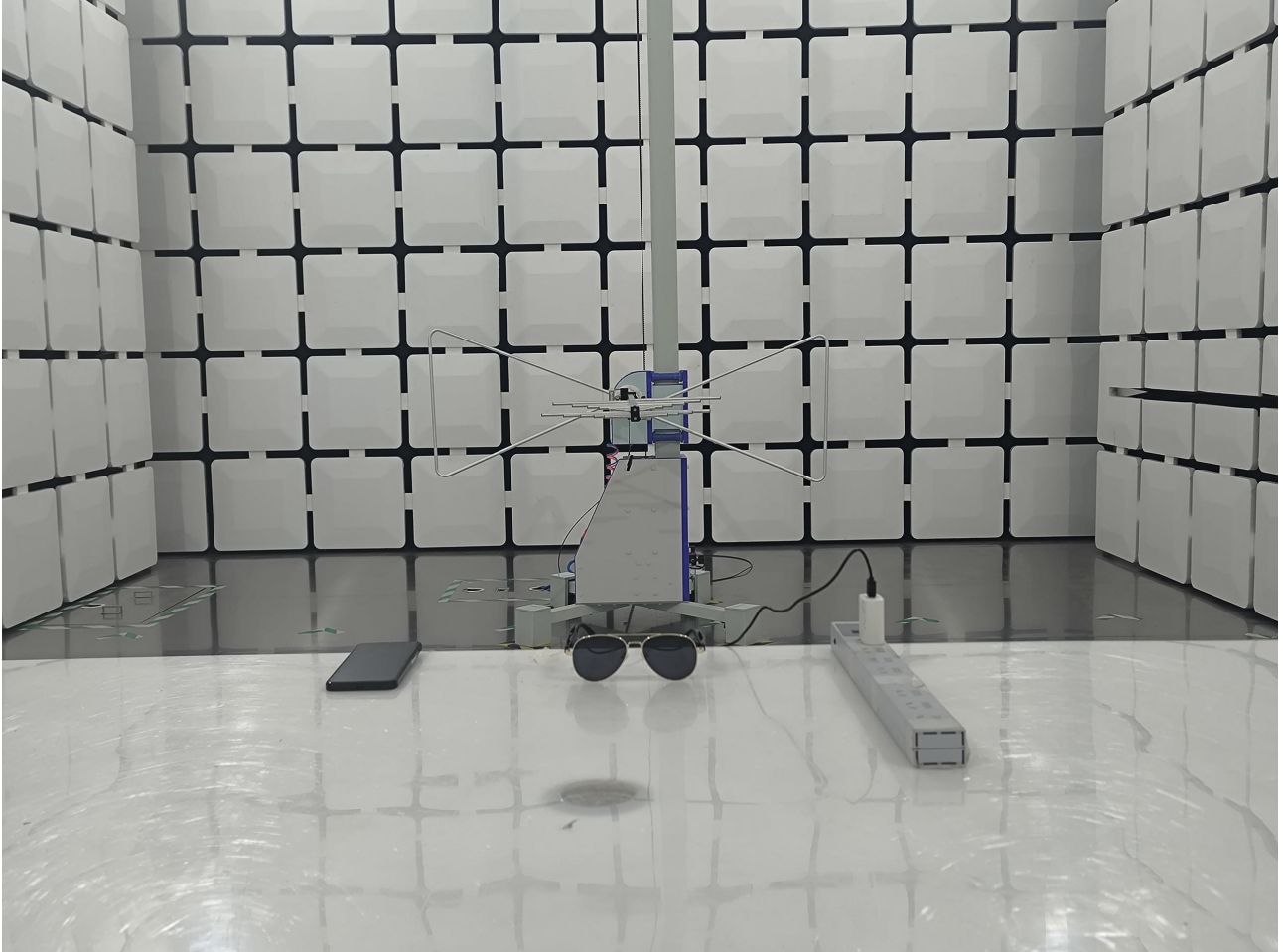
Radiated Emission Test View 1
