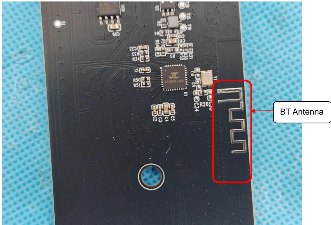
INTERNAL VIEW OF EUT(FIGURE 29)
