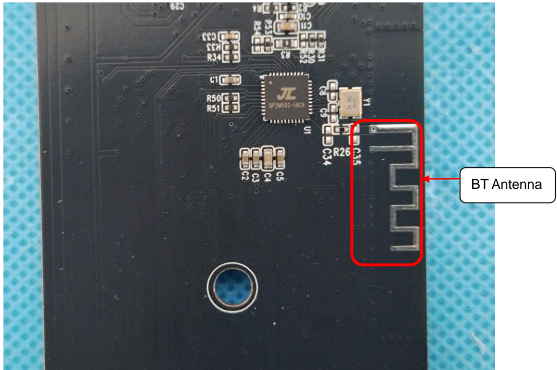
INTERNAL VIEW OF EUT(FIGURE 23)
