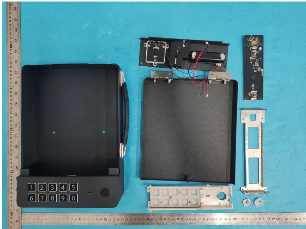
OPEN VIEW OF EUT(FIGURE 8)
