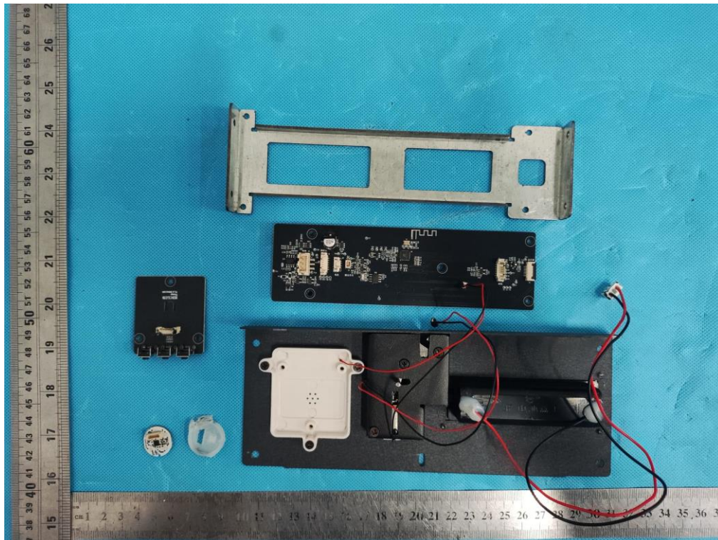
OPEN VIEW OF EUT(FIGURE 11)
