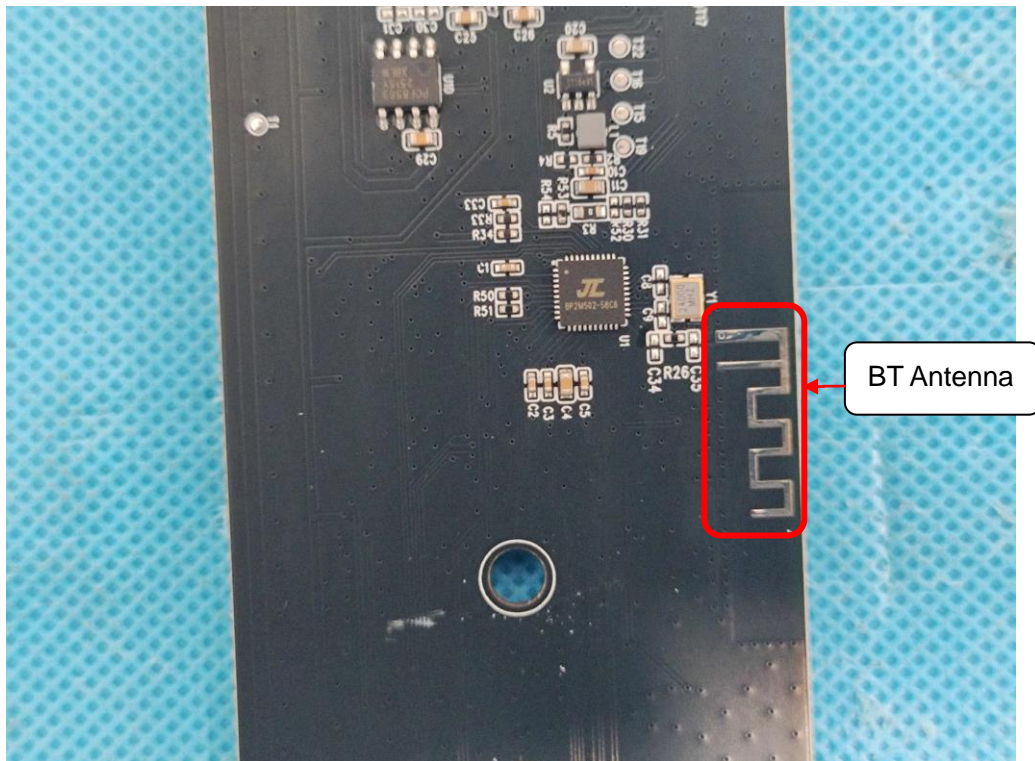
INTERNAL VIEW OF EUT(FIGURE 11)
