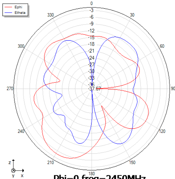
Phi=0 freq=2450MHz
