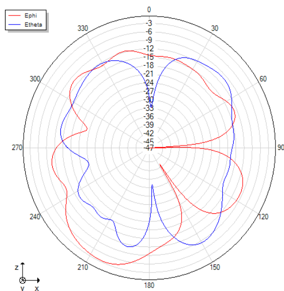
Phi=0 freq=2420MHz
