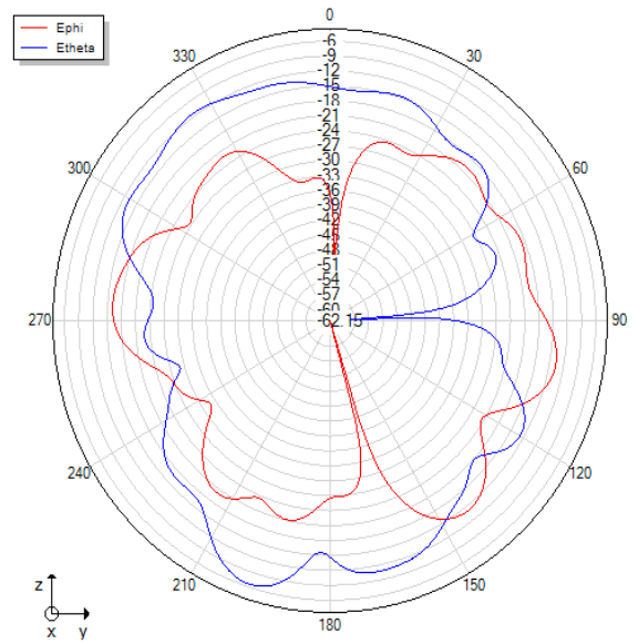
Phi=90 freq=2470MHz
