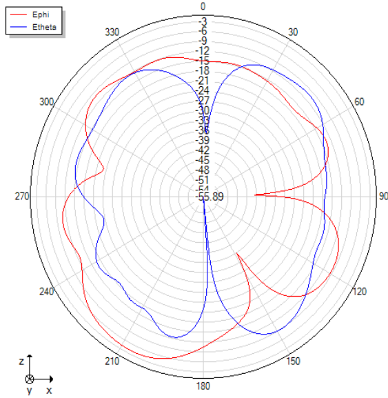
Phi=0 freq=2430MHz
