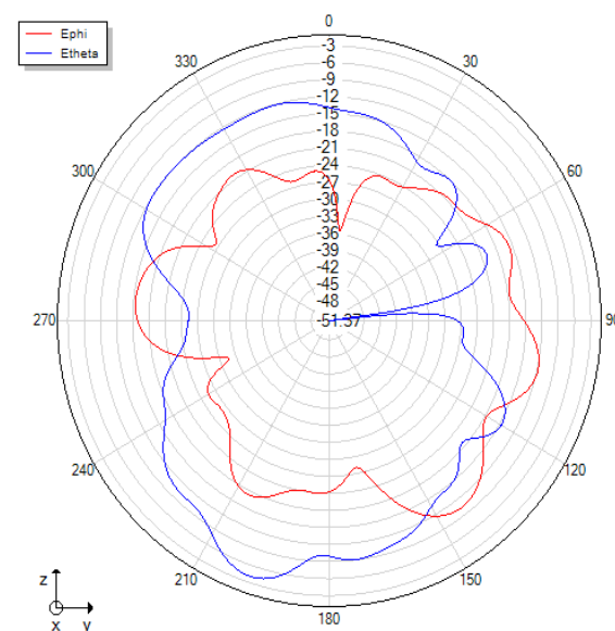
Phi=90 freq=2410MHz
