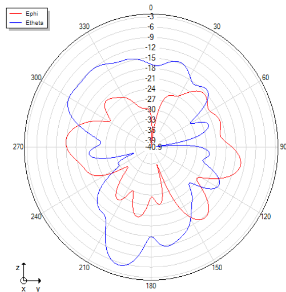
Phi=90 freq=2500MHz
