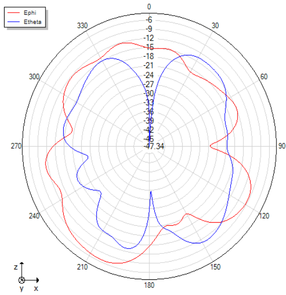
Phi=0 freq=2470MHz
