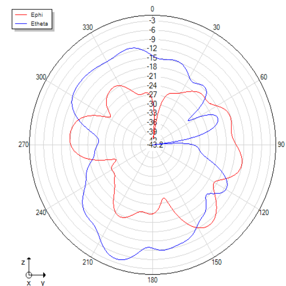
Phi=90 freq=2420MHz
