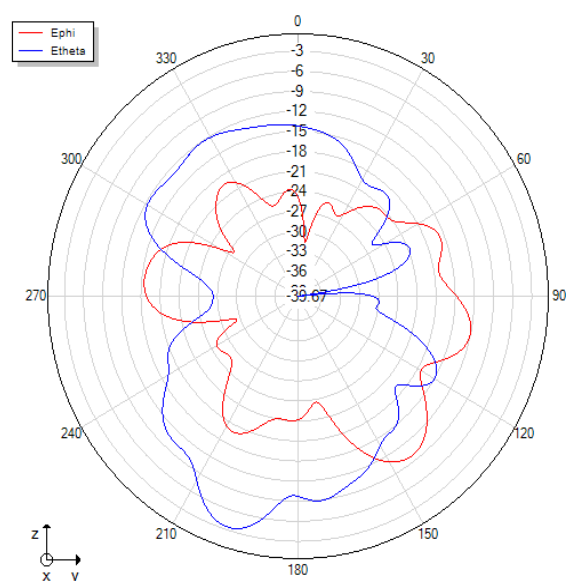
Phi=90 freq=2400MHz
