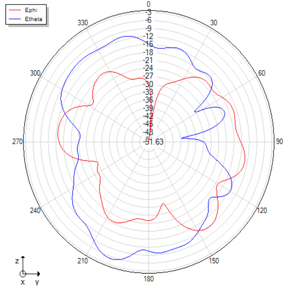
Phi=90 freq=2430MHz
