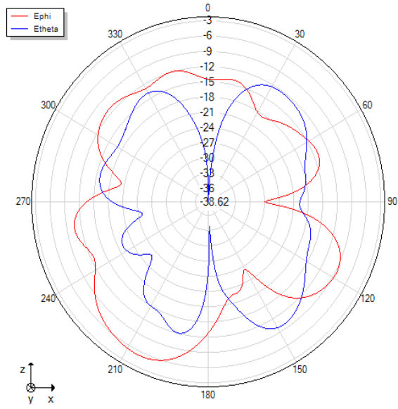
Phi=0 freq=2460MHz
