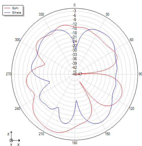
Phi=0 freq=2410MHz
