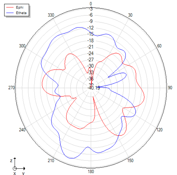
Phi=90 freq=2450MHz
