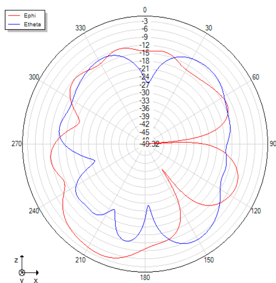
Phi=0 freq=2400MHz
