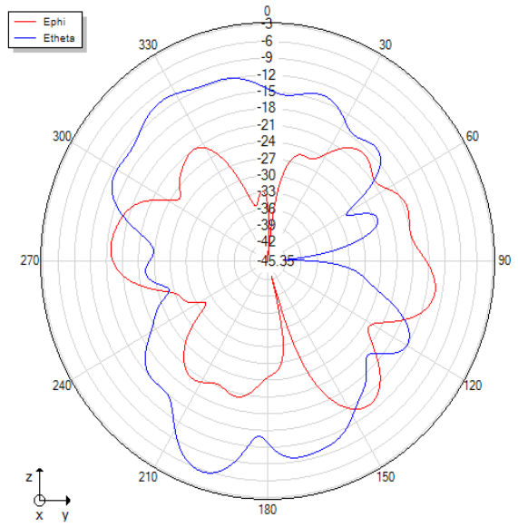
Phi=90 freq=2460MHz
