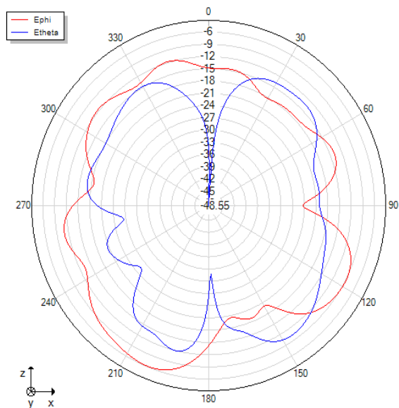
Phi=0 freq=2480MHz
