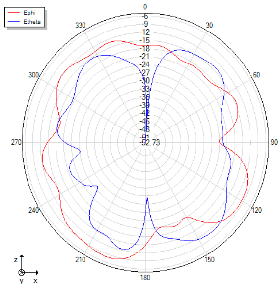
Phi=0 freq=2500MHz
