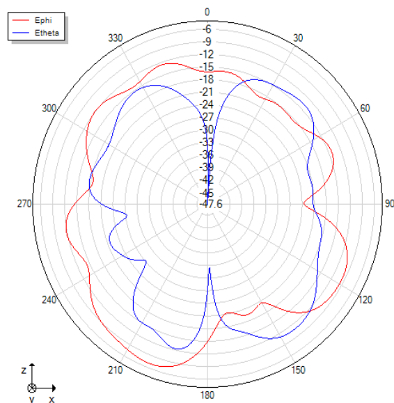
Phi=0 freq=2490MHz
