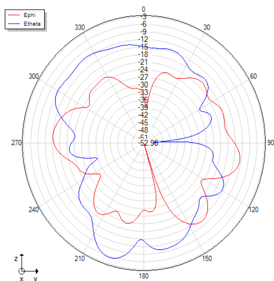
Phi=90 freq=2480MHz
