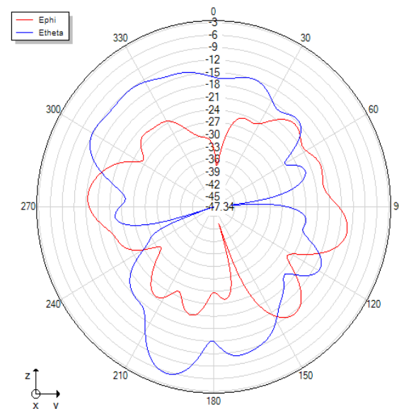
Phi=90 freq=2490MHz
