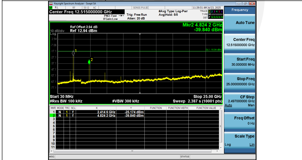
2_Spurious Emission_NVNT_ANT1_User_2412
