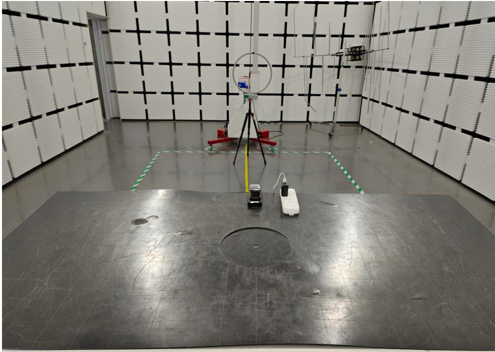
Spurious Radiation Emissions Test (<30M)
