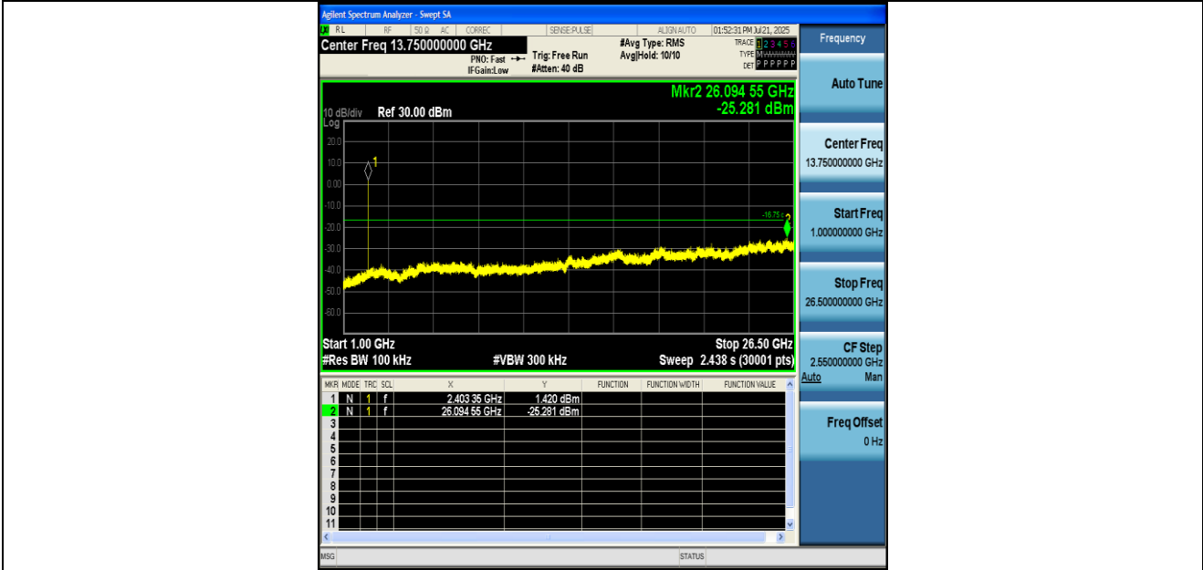
SRD-Ant1-2403-1000~26500-PASS
