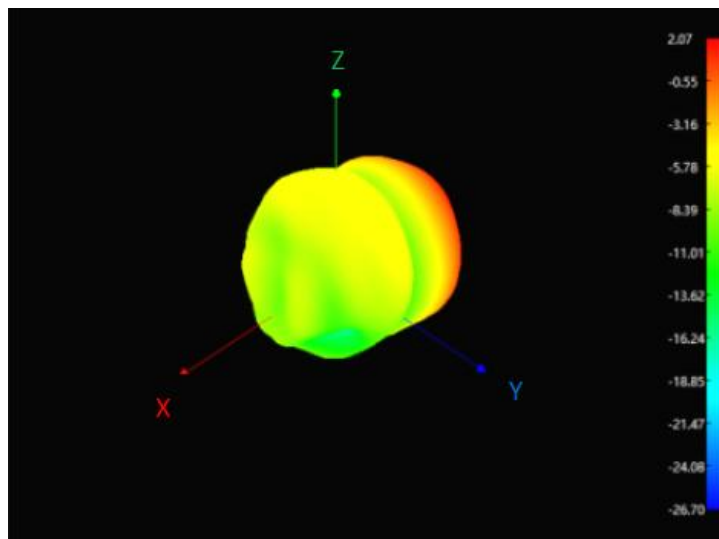
2440MHz 3D
