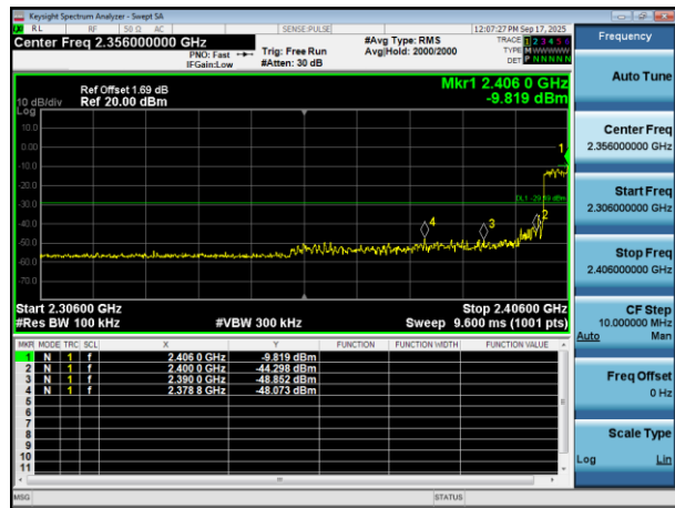
Band-edge Emission
