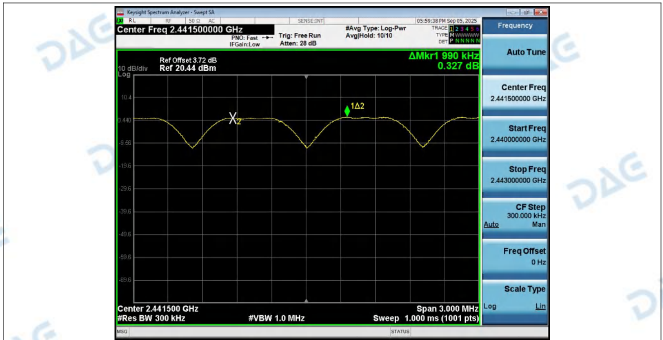
Carrier_Frequencies_Separation_(Hopping)_NVNT_ANT1_1-DH5_Hopping
