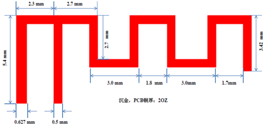
Antenna Dimension for ESP33-WROOM-32
