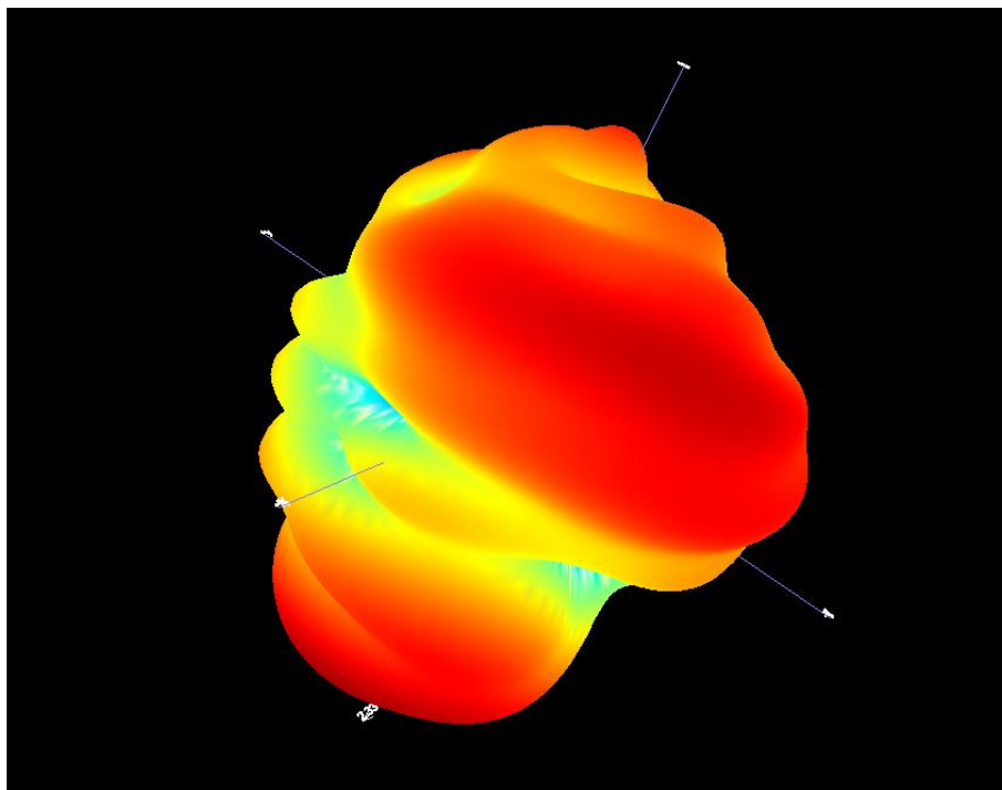
B1.1 3D Pattern for 2400MHz
