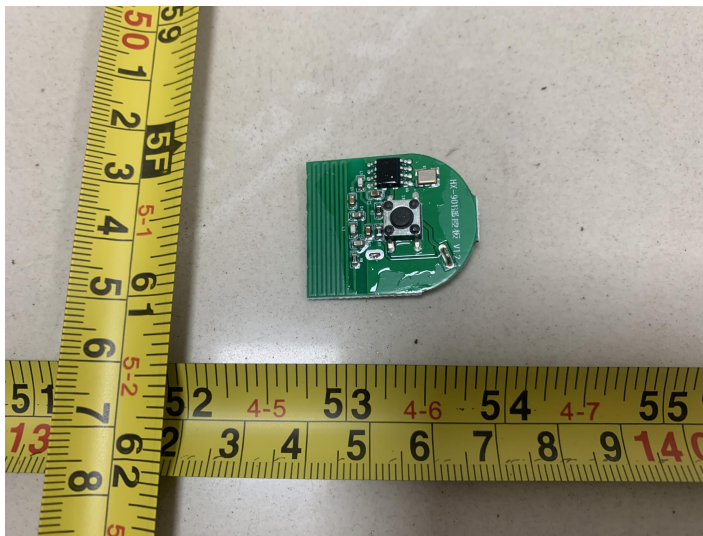
Antenna Gain:0dBi
