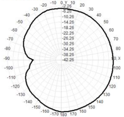
Total(H-XY), Max=-2.62dBi, CirD=19.01
