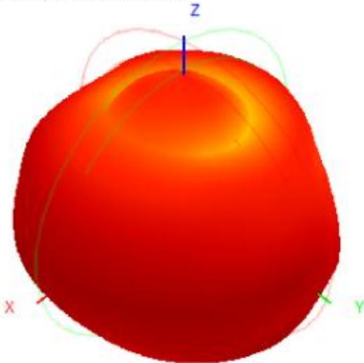
2500.0MHz H+V, Eff: 24.0%
