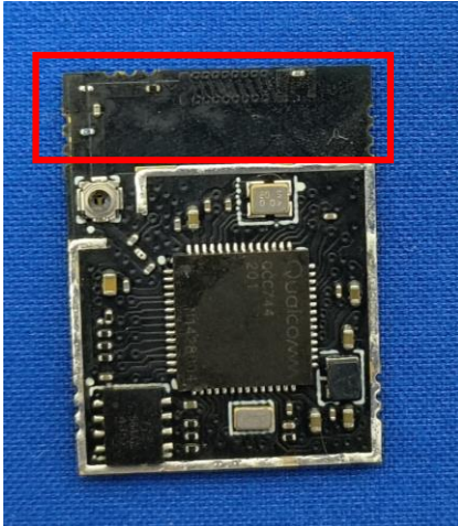
PCB Antenna
