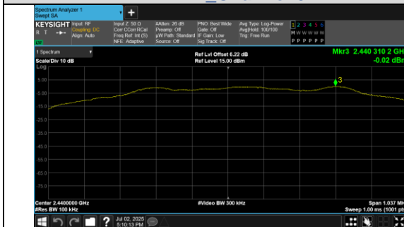
In-Band Reference Level BLE 1M_Channel 19
