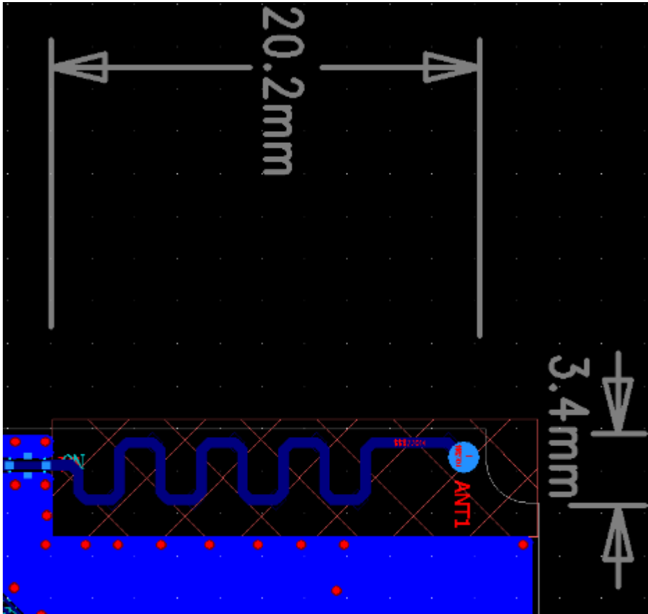
H0401 Antenna Photo & Length
