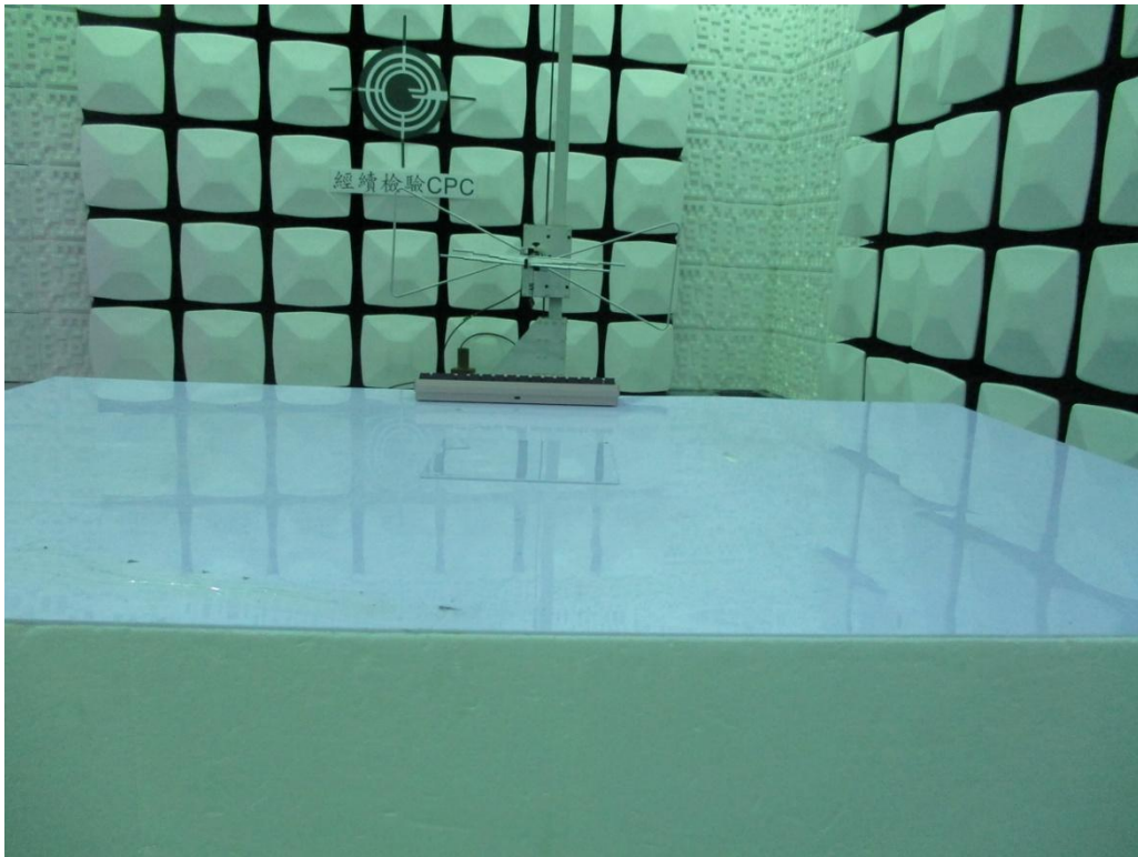
Setup Photo FCC ID: 2BQVO-KL65-68
