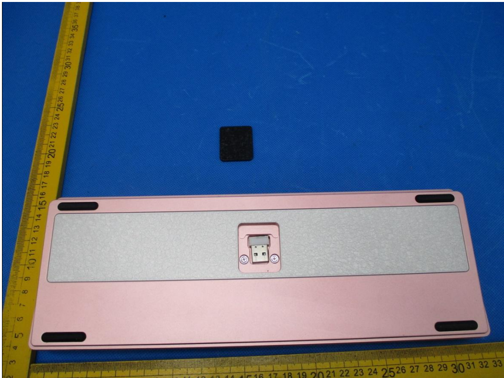
Internal Photo FCC ID: 2BQVO-KL65-68
