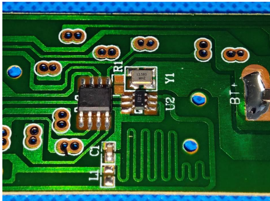
(a) Antenna
