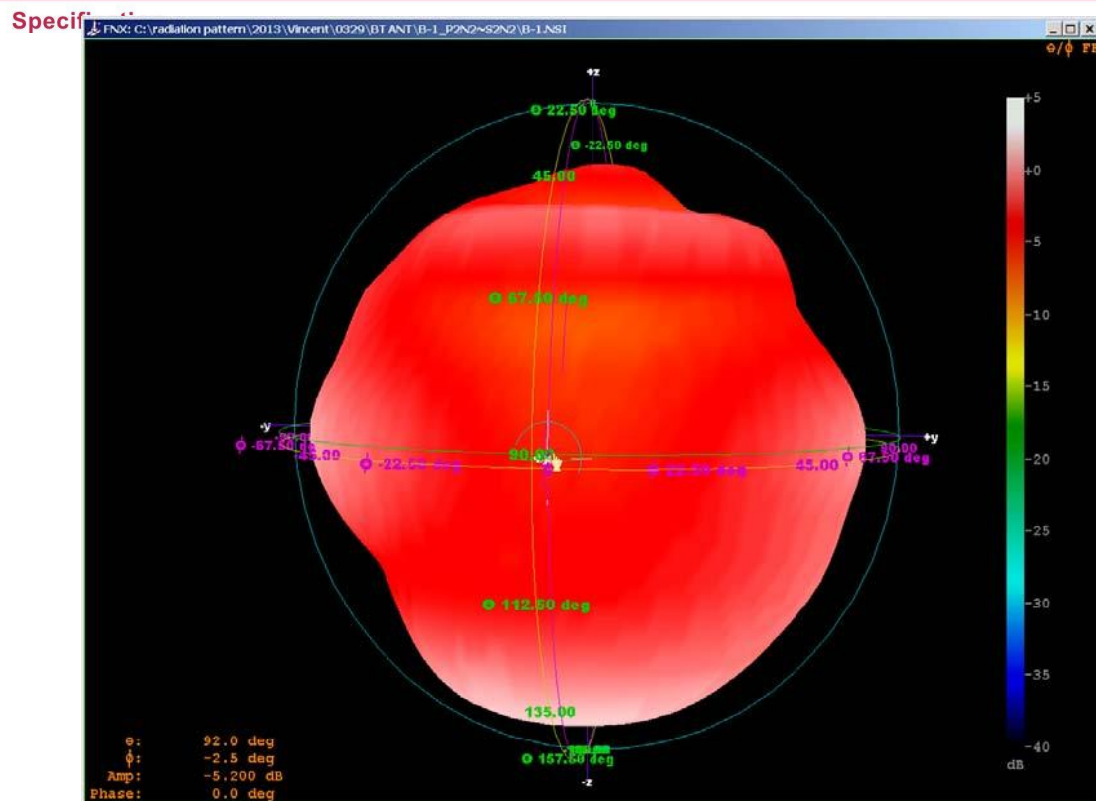
3D radiation pattern diagram
